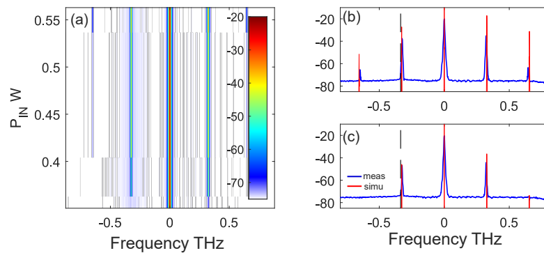
Figure 6.5 – (a) 2D plot of the spectra as a function of P_{in} for a finesse of about 105. (b) and (c) two examples of measured spectra (blue) and simulated spectra, for P_{in} = 0.53 W and P_{in} = 0.35 W respectively. The black dashed line marks the central position of the filter. The parameters of the simulation are listed in the caption of Fig. 6.1.
