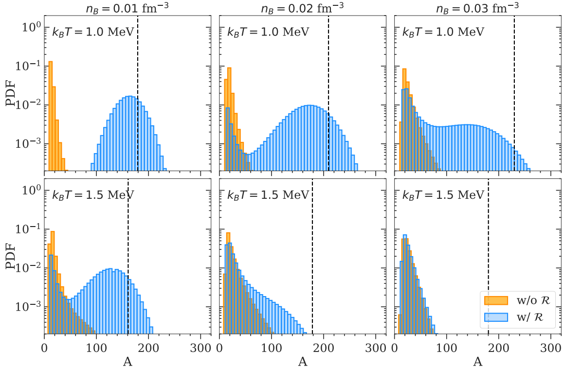
Figure 4.33: Same as Fig. 4.32 but for the ion mass number A . See text for details.
