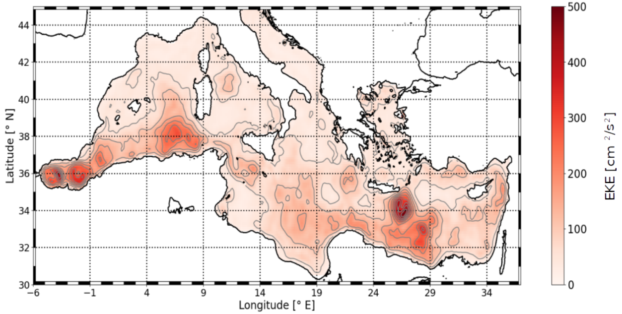
Figure 1.7: Eddy kinetic energy (EKE) from 2000 to 2015 using altimetry in geostrophic approximation, gray lines are 50\text{cm}^2.\text{s}^{-2} isolines.
