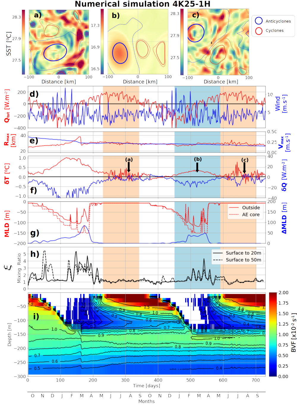
Figure 4. Simulation 4K25-1H from Table 1. (a) SST snapshot in the first summer, (b) in the second winter, (c) in the second summer, contours are AMEDA eddy detections. The initial anti-cyclone is highlighted by a thicker line. (d) Net heat flux (red) and wind speed (blue). (e) R_{max} (red) and V_{max} (blue) from AMEDA. (f) SST anomaly index \delta T (red) and heat flux anomaly \delta Q (blue). (g) Mixed layer inside-eddy (dashed red) and outside-eddy (continuous red), mixed layer anomaly is in continuous blue. (h) Differential mixing ratio \xi defined in Eq.13 with h = 20m (solid) and h = 50m (dashed line). (i) Inside-eddy stratification evolution shown with Brunt-Vaisala frequency (scale factor 100) ; contours are overlaid with 0.001 s^{-1} intervals and negative values are blanked. On panels d-h, summer periods are indicated by light red shades, winter by a light blue shade.
