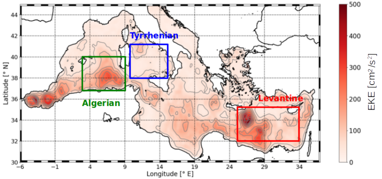
Figure A.2: Mean Eddy Kinetic Energy map of the Mediterranean Sea, showing the three eddying regions chosen to investigate climatological eddy impact on MLD.
