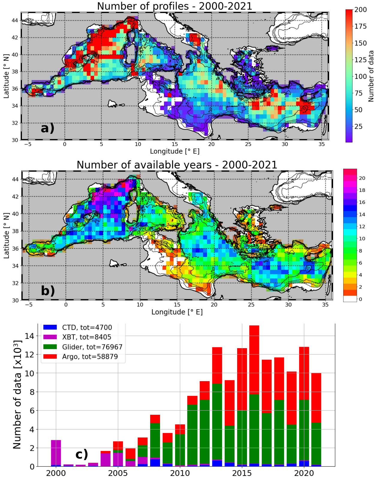
Figure 2.5: (a) Number of available measurements per 0.5° bins; (b) number of years with available measurements per 0.5° bins; (c) yearly histogram of in situ profiles distinguishing different data types.
