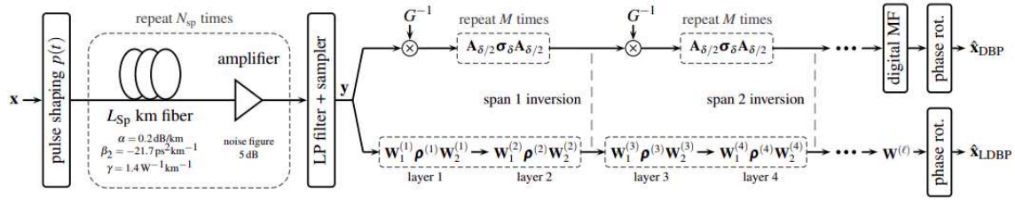
Figure 3.9: The system model shown in [49]. The top processing branch depicts DBP implemented via the SSFM, while the bottom branch shows the LDBP approach obtained by "unrolling" the SSFM. The LP and MF blocks represent the low-pass and matched filters, respectively. LDBP performs similarly to DBP in the absence of parameter optimization via deep learning and when the same number of steps/layers are used.
