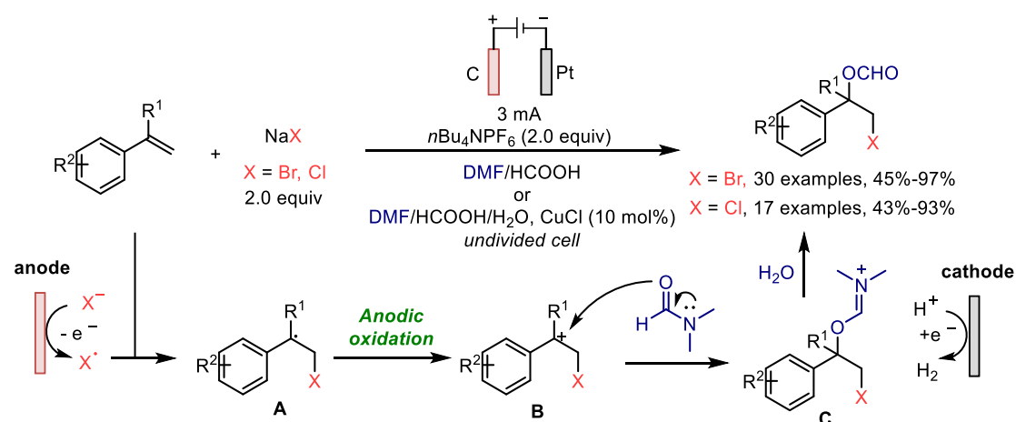
Scheme 74. Electrochemical oxidation halogenation-formyloxylation of alkenes.
