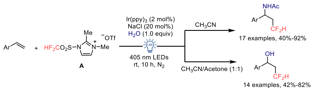
Scheme 34. Visible-light-induced Difluoromethylation of Alkenes by using Difluoromethylsulfonamide Imidazolium Salt.
