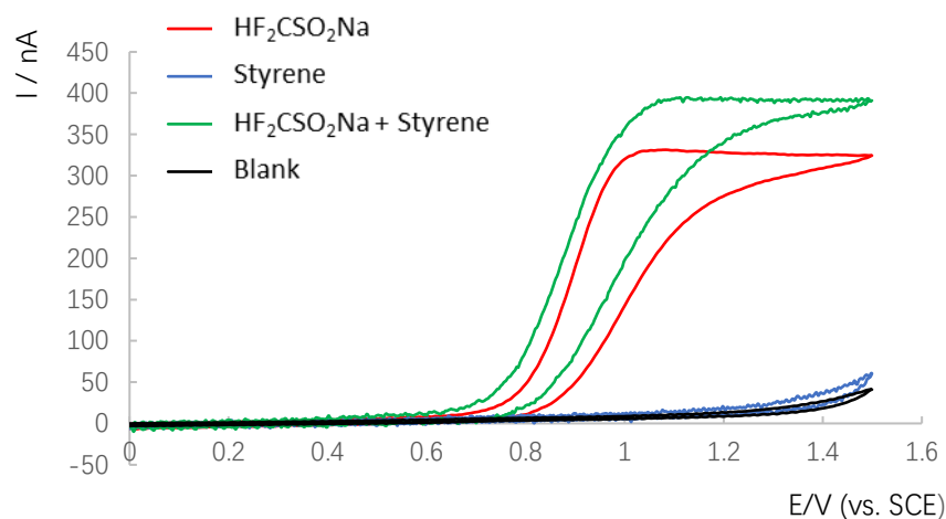
Figure 15. CV curve for a solution of 0.01 M \text{HF}_2\text{CSO}_2\text{Na} /0.02 M Styrene and 0.05 M n\text{Bu}_4\text{NBF}_4 in Acetone on a Pt working electrode ( d = 0.1 mm), Pt wire ( d = 1 mm) auxiliary electrode, SCE reference electrode under a scan rate of 0.1 V/s ranging from 0 V to 1.5 V in oxidation. Following IUPAC CV plotting convention.
