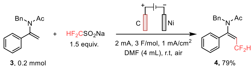
Scheme 48. Optimal conditions.
