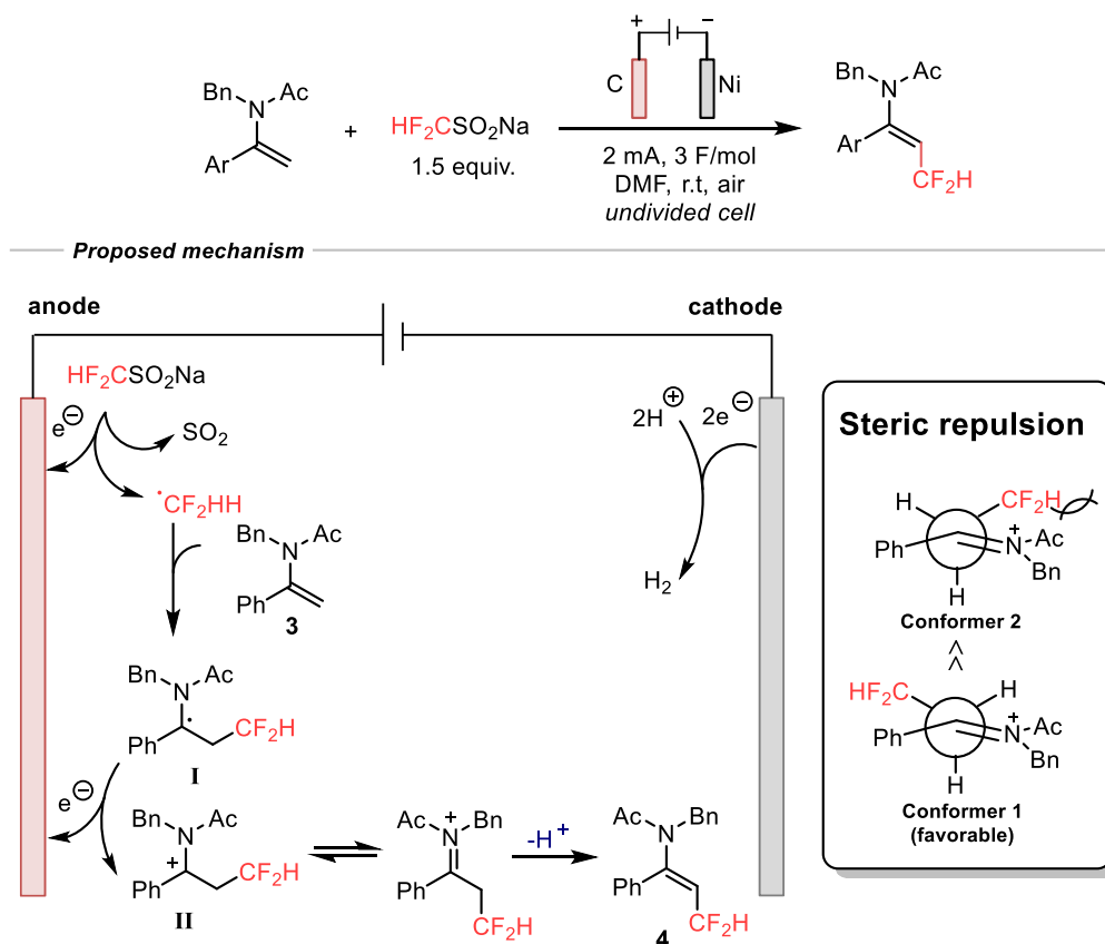
Scheme 52. Proposed Mechanism.
