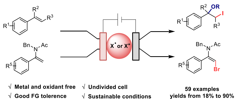
Scheme 100. Electrochemical halogenation of enamides.
