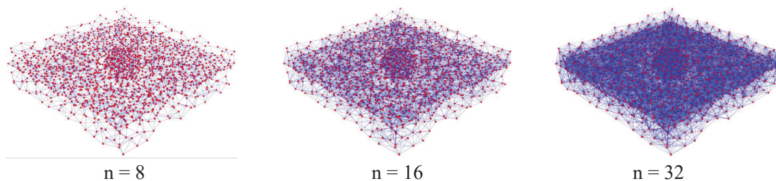
FIGURE 7.7: Influence of the neighborhood size n over the topology of the graph.
