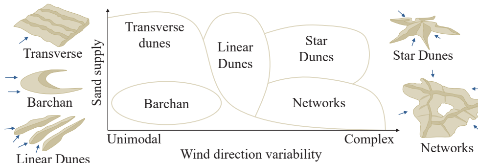
FIGURE 4.3: Different types of dunes in relation to the variability of wind direction and available sand supply. Figure inspired from Livingstone et al. 1996.
