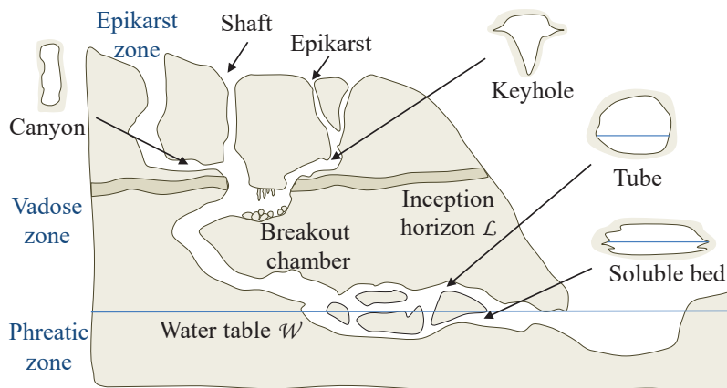
FIGURE 7.2: Idealized cross-section through a complex underground cave network.
