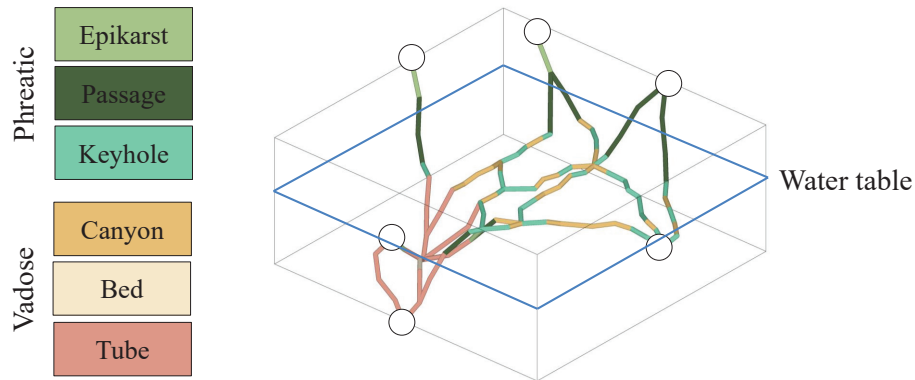
FIGURE 7.15: Classification of tunnel types on a generated network.
