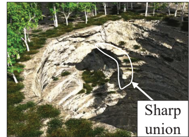
FIGURE 5.6: Union operator for carving a karstic tunnel.
