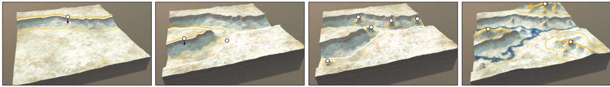
FIGURE 2.12: Gradient-domain authoring (Guérin et al. 2022) offers powerful tools to the user, where elevation (white) and gradient (yellow) constraints on points and along curves can be placed to create different landforms such as peaks, table mountains, crevasses and canyons.
