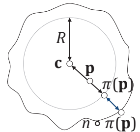
FIGURE A.3: Perturbed sphere primitive.
