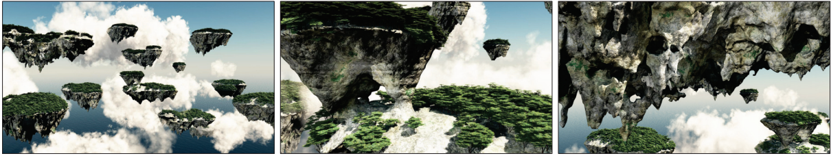
FIGURE 6.23: The floating islands were created by combining implicitized heightfields; an erosion operator was then added to the construction tree to produce a precise stratification, and we finally carved some tunnels and caves into the bedrock of one island by applying the Invasion-Percolation algorithm. Individual islands are between 300m and 600m wide and were placed manually in the scene, for a total of 6mb in memory.
