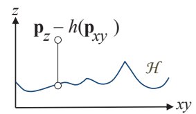
FIGURE 6.6: Vertical distance to a heightfield.
