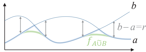
FIGURE 5.8: Smooth union between two functions a and b .
