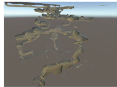
FIGURE 2.23: Rectilinear karstic network generated by Franke et al. 2022.
