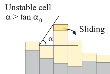
FIGURE 2.14: Granular material stabilization process.
