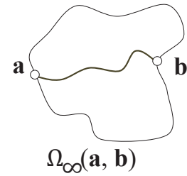
FIGURE 7.12: Geometric representation of \Omega_\infty .
