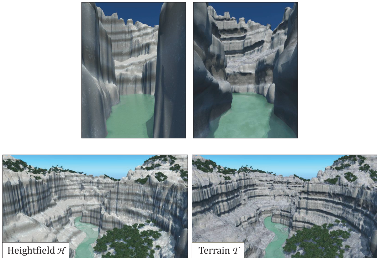
FIGURE 6.14: A comparison between raw data (with a resolution of 1m per pixel) of The Mystery Canyon in the Zion National Park, Utah, and the outcome of the amplification process. Volumetric features occupy 20% of the terrain's surface area.
