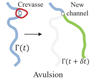
FIGURE 3.13: Avulsion process in a channel.
