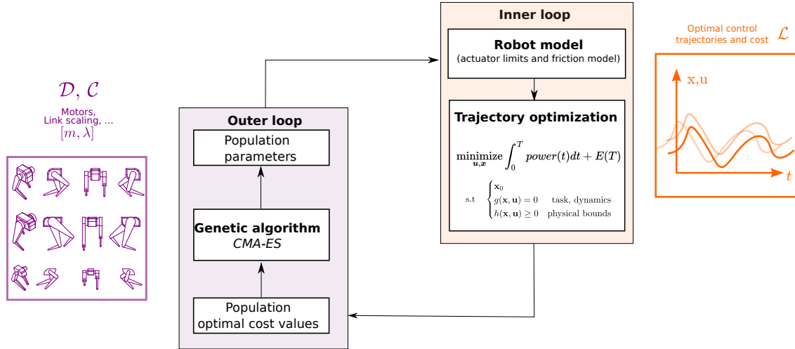
Figure 31: Co-design approach and the bi-level formulation
