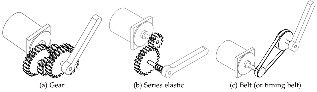
Figure 15: Transmission types
