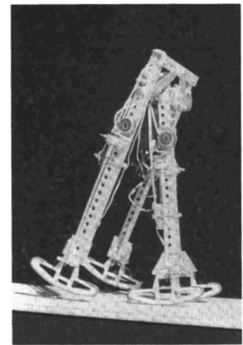
(b) Planar passive walker by Tad McGeers
