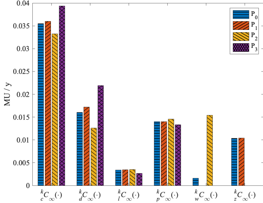
Figure 5.8 – Values of {}^c C_\infty(\cdot) , {}^d C_\infty(\cdot) , {}^l C_\infty(\cdot) , {}^p C_\infty(\cdot) , {}^w C_\infty(\cdot) , and {}^z C_\infty(\cdot) under each of the considered policies in the case of the setup \mathcal{D}_1 .
