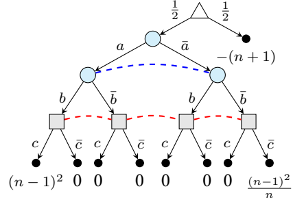
Figure 3.8: Game G_{-\sqrt{n}}
