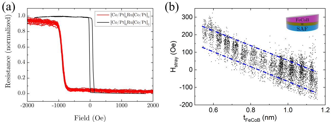
Figure 3.2: a) Field hysteresis loop of two devices from different samples, fabricated with a SAF using different Co/Pt repetitions in the top SAF block, [\text{Co/Pt}]_6/\text{Ru}/[\text{Co/Pt}]_3 in red and [\text{Co/Pt}]_6/\text{Ru}/[\text{Co/Pt}]_2 in black. b) Stray field dependence with the FeCoB reference layer thickness. The critical thickness of \approx 1\text{nm} results in a mean zero offset with a dispersion of \pm 50\text{Oe} . The full stack of this sample is Ta(22) / FeCoB(0.8) / W(2) / Pt(7) / SAF / FeCoB(0.5-1.15) / MgO(2.3) / FeCoB(0.9-1.9) / W(2) / Pt(5) / Ru(3) / Ta(150)
