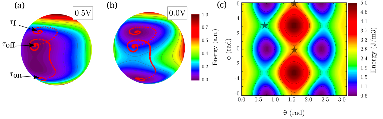
Figure 2.19: Representation of the energy density of the system for different applied voltages and the magnetization trace during switching in red for a pulse of 1ns. a) 3D Energy landscape at 0.5V, with t_0 being the time of pulse initialization, t_{off} the time when the pulse is turned off, and t_f the end of the simulation. b) 3D Energy landscape at 0V. c) 2D energy landscape at 0V with saddle points marked by black stars.
