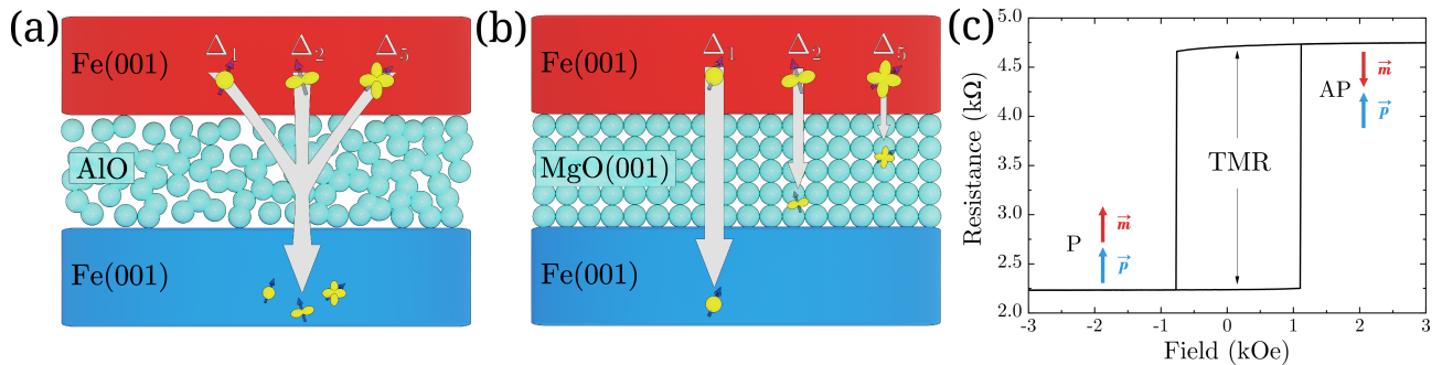
Figure 1.2: Schematic of orbital symmetry tunneling characteristics in a tri-layer using a) Amorphous AlOx compound and b) Crystalline MgO with lattice [001]. c) Example of a magnetic hysteresis loop showing the TMR signal and the distinction between the two stable states P and AP.
