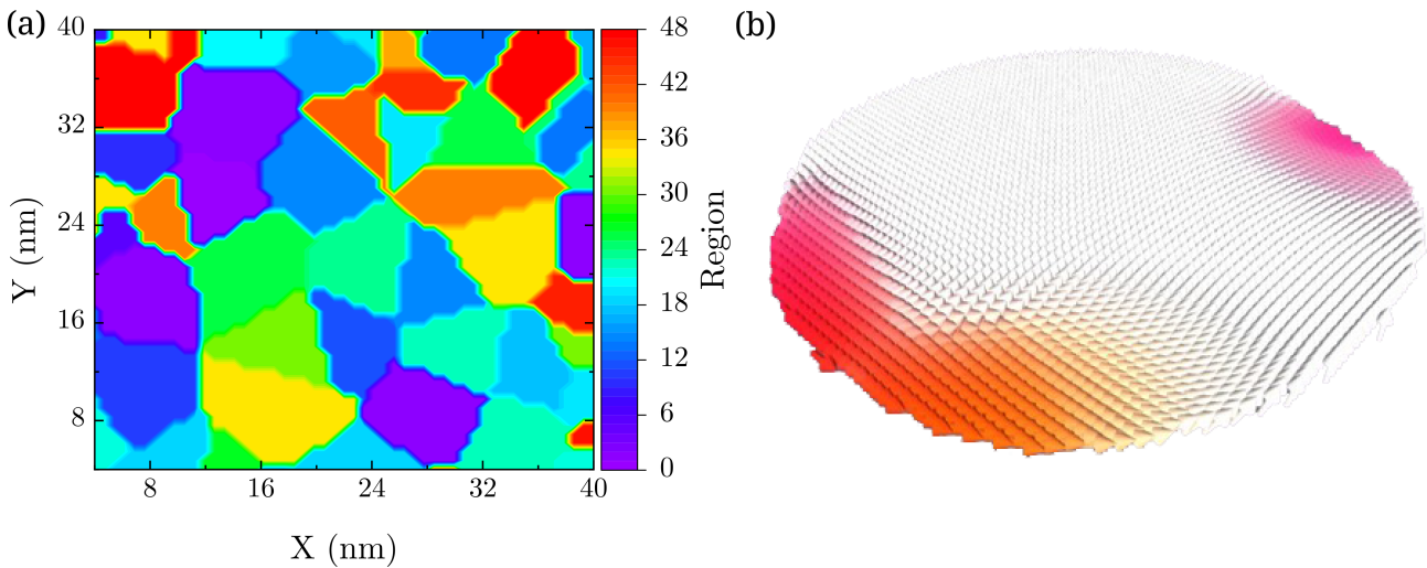
Figure 2.25: a) Region definition within MuMax3 environment in which each one has a K_1 that follows a normal distribution with a 10% variance. b) The magnetization state of a layer using a tessellated K_1 structure, with m_z lower than 1 without any external fields applied.
