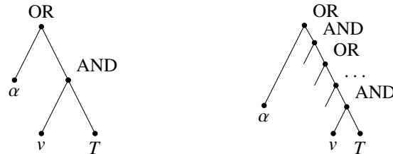
Figure 6.2: Shallow pruning vs. deep pruning; T can be pruned (shallowly or deeply) if v \preceq \alpha .
