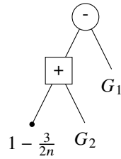
Figure 4.2: An EFG with two 3-colouring subgames G_1 and G_2 .
