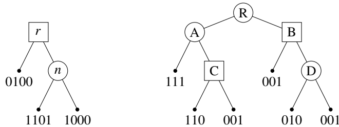
Figure 6.1: Two AND-OR DAGs with partially ordered values.
