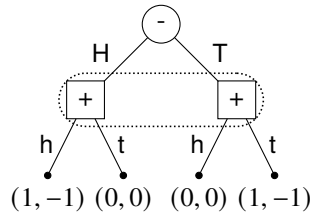
Figure 3.3: Matching Pennies.
