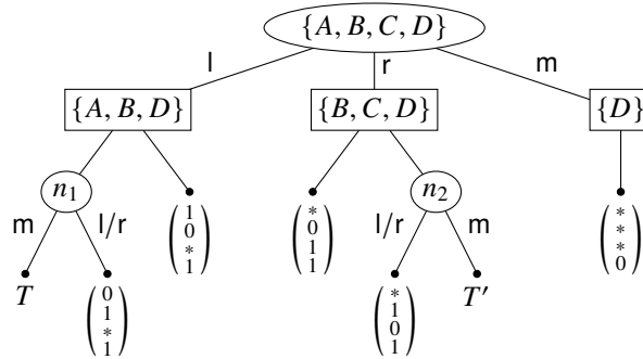
Figure 6.9: An information-revealing CGII, where T denotes an unspecified subtree in which MIN of type D can force a loss for MAX and T' denotes another unspecified subtree in which MAX can force a win.
