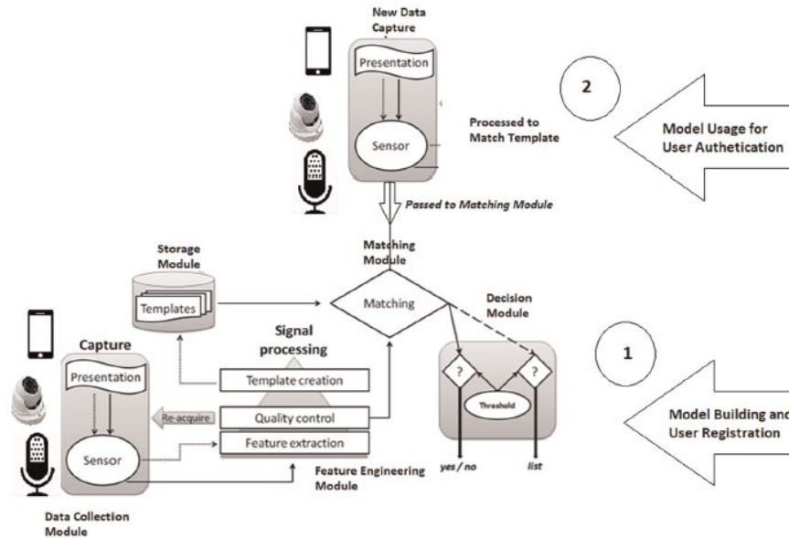
FIGURE 2.6: Behavioral biometric model [Sharma and Elmiligi, 2022].
