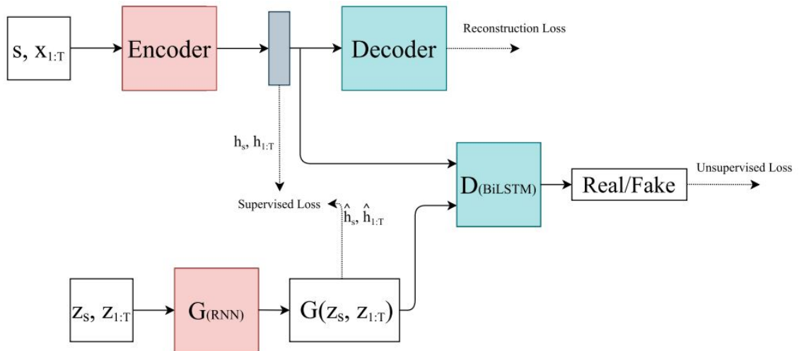
FIGURE 4.2: TimeGAN architecture.
