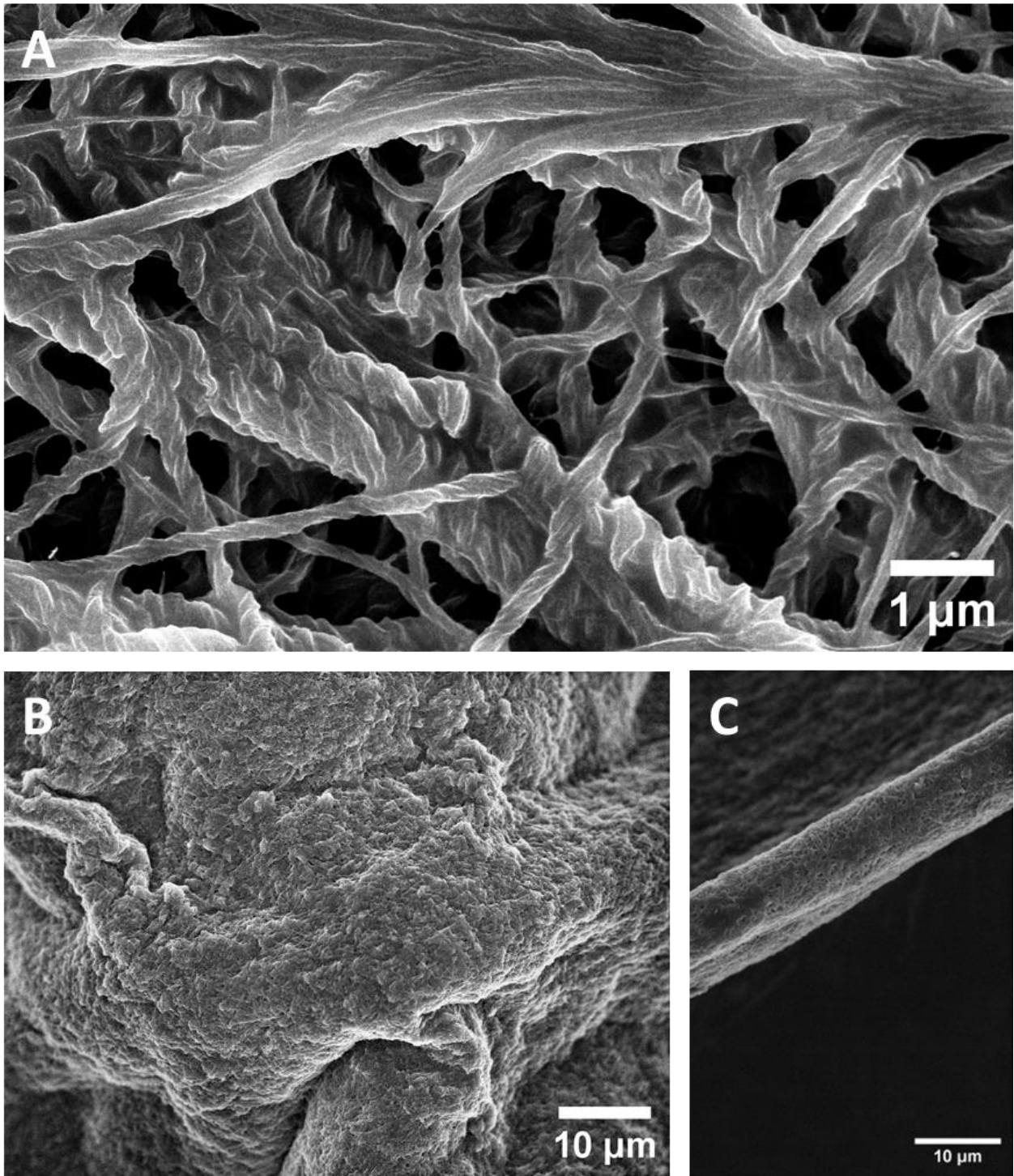
Figure 169: SEM images of Collagen I membranes at high (A) or low (B&C) magnification, A) Collagen fibril bundling fibers up to a few \mu\text{m} diameter, B) membrane ruffles, and C) edge view of a membrane.
