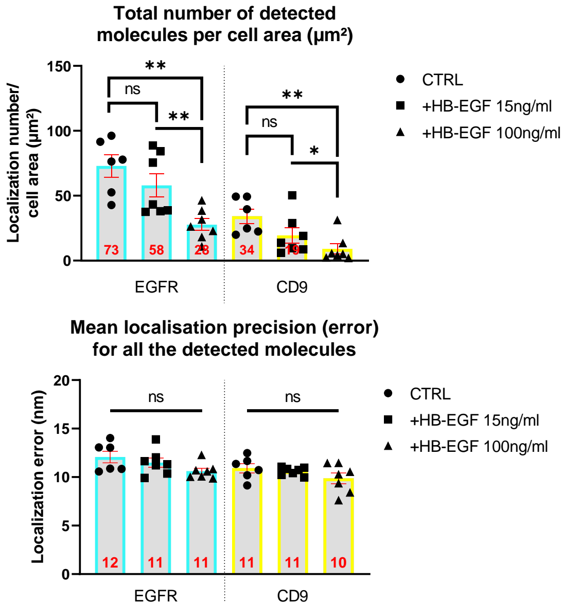
Figure 115: Top, total EGFR and CD9 localization count per images, and bottom, average localization error from molecule fits for mPECs grown on glass coverslips and labeled for EGFR (Cyan, labeled with CF568) & CD9 (Yellow, labeled with Dylight 650) with control cells, cells stimulated with 15 ng/ml or with 100 ng/ml HB-EGF ( n=6 , error bars are SEM, stars from t-test).
