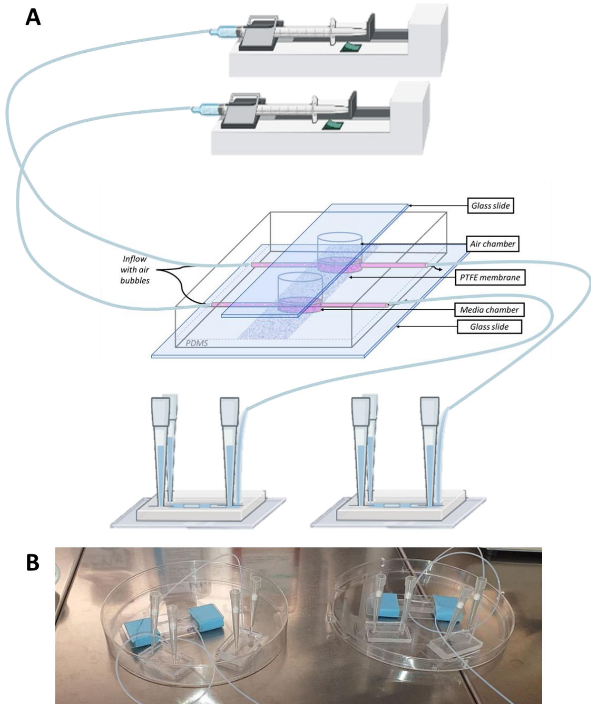
Figure 55: A) Scheme of syringe driven perfusion in line with bubble trap. When bubbles reach the trap chambers they are trap and ruptured on the PTFE membrane and reservoir. The traps are then connected to the systems. B) picture of the assembly under the hood.
