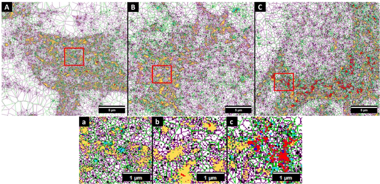
Figure 127: A, B, & C) 2 color dSTORM super resolution reconstructed images of mPECs labeled for EGFR (Magenta, labeled with CF568) & CD9 (Green, labeled with Dylight 650) processed with Voronoi tessellation (overlapping clusters are red, isolated clusters are blue, close clusters are yellow), red squares indicate region of interest enlarged in a, b, & c, A&a) are control cells, B&b) are cells stimulated with 15 ng/ml HB-EGF, C&c) are cells stimulated with 100 ng/ml HB-EGF (pixel = 20 nm, magnification 100X).
