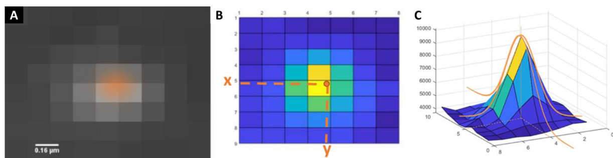
Figure 104: A) Gray level image of a blinking event, B&C) representation of the raw pixel matrix in 2D with localization x,y determination from gaussian fits, the orange spot in A) represents the molecule localization and the spot width reflects the localization precision.
