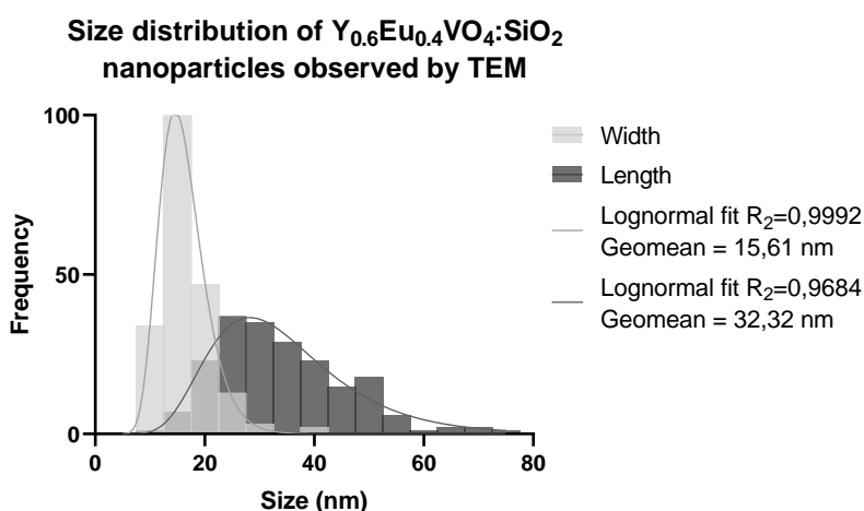
Figure 134: Size distribution of silica-coated Y_{0.6}Eu_{0.4}VO_4 nanoparticles obtained from TEM images (200 individual nanoparticles were analyzed).
