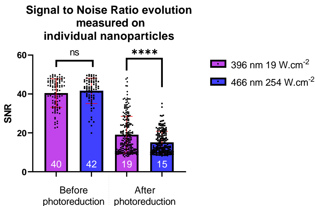
Figure 150: Individual nanoparticles SNR extracted from photoreduction experiments using either 396 or 466 nm excitations ( n=5 images each \sim 20 NPs per image, error bars are SEM, stars indicate significant Kolmogorov-Smirnov t -test).
