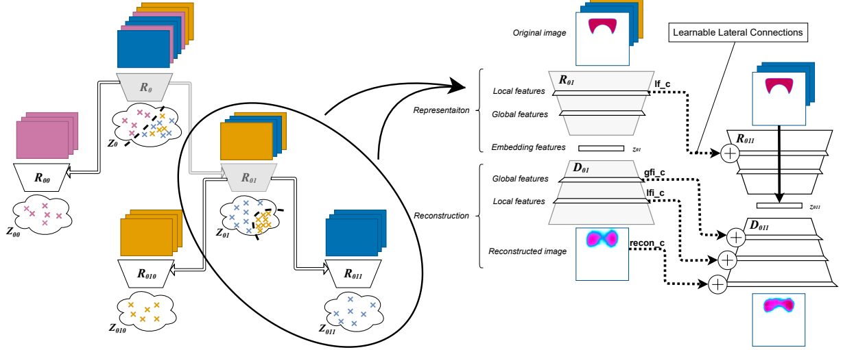
Figure 5.3.: Overview of HOLMES architecture used in the work presented in Etcheverry et al. [•3]. (Left) Each module uses a VAE [137] as the base architecture, where the embedding \mathcal{R}_i is coupled to a decoder \mathcal{D}_i ( \mathcal{D}_i is not shown on the left panel for readability). All non-leaf node VAEs are frozen as well as their incoming lateral connections (light grey). The leaf nodes are incrementally trained on their own niches of patterns (represented as colored squares above the embeddings) defined by the boundaries fitted at each node split (curved dotted lines in each BC space, represented as clouds). (Right) \mathcal{R}_{011} is trained to encode new information in a latent representation z_{011} (plain vertical arrow) by learning to reuse its parent knowledge via the lateral connections (dotted arrows).
