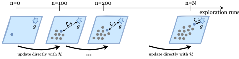
Figure 3.20.: Non-parametric learning
