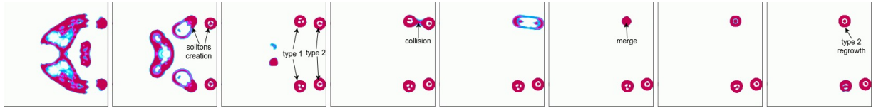
(g) Here, solitons seem to co-exist into two different shape modes , with collision leading to merge and regrowth in the second mode
