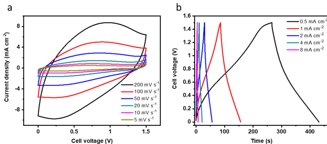
Figure 2.22: a. CV curves at different scan rates and b. GCD curves at different current densities of all-solid-state MSC device tested using SiWa-doped TEAH/TFPI electrolyte at 1.5 V.
