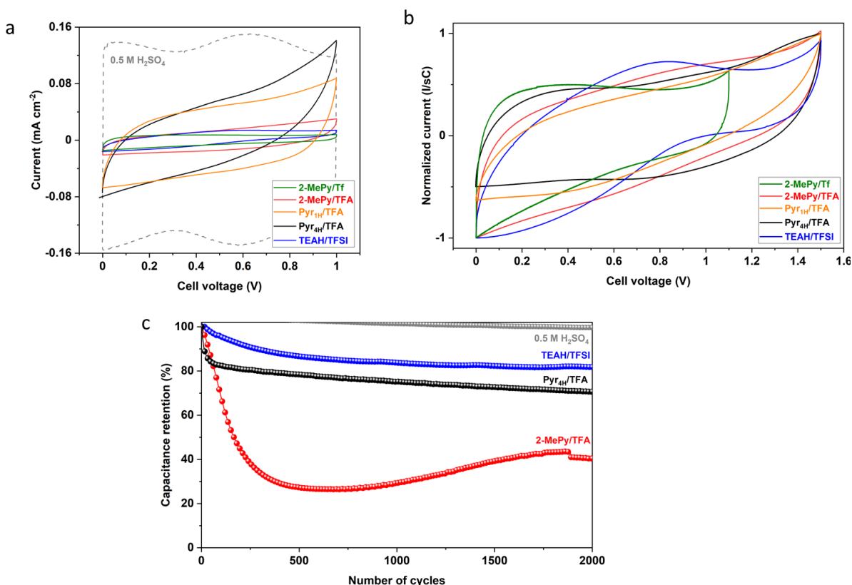
Figure 2.7: a. Cyclic voltammety (CV) curves of RuO 2 on interdigitated flat Au substrates tested in different PILs and their comparison with 0.5 M H 2 SO 4 (scan rate of 100 mV s -1 ); b. Normalized CVs of RuO 2 in PILs at a scan rate of 100 mV s -1 ; c. Cycling stability performance of RuO 2 MSCs in different electrolytes at 1 mA cm -2 .
