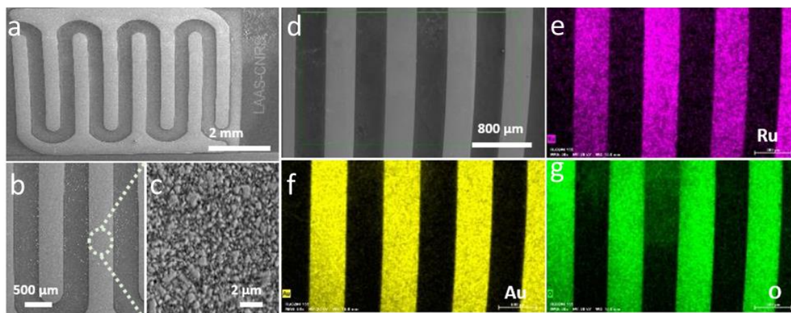
Figure 2.3: SEM images at different magnifications (a-d). EDS elemental mapping of \text{RuO}_2 deposited on interdigitated flat Au current collector (e-g).
