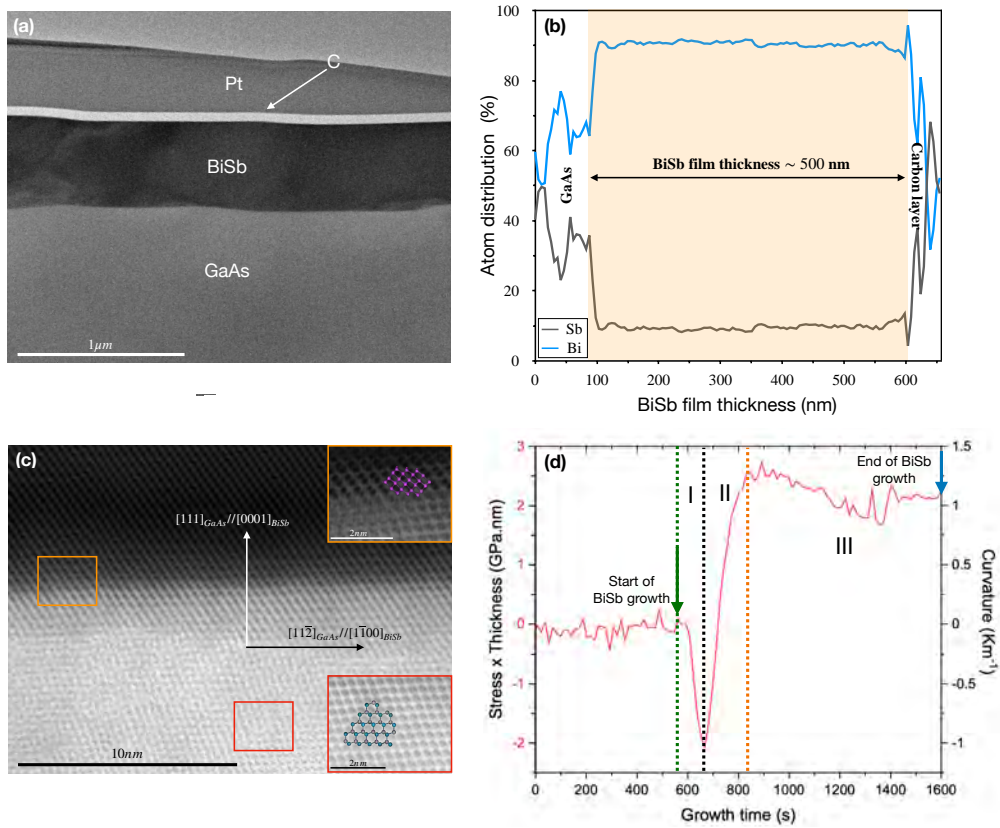
Figure 5.9: Cross sectional characterisation of a 500 nm-thick \text{Bi}_{0.9}\text{Sb}_{0.1} layers. (a) TEM image of the BiSb/GaAs interface. (b) Distribution of Bi and Sb atoms in the cross-section. (c) High-resolution TEM image taken along the [1\bar{1}0] zone axis of the GaAs. The red and orange inset images are a zoomed image of the zone indicated by a red and orange square, respectively. Both insets show the side views of the crystal structure of GaAs and BiSb grain. Bi, As and Ga are represented by pink, blue and gray, respectively. (d) Stress \times thickness and associated curvature as a function of growth time measured on a 90 nm-thick sample. The green and blue arrows indicate the start and end of BiSb growth, respectively.
