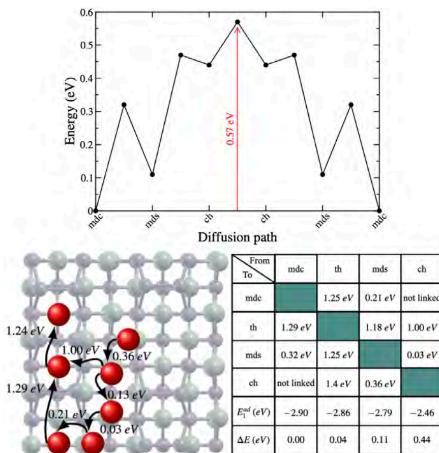
Figure 4.20: (Top) The minimum energy path calculated for Bi atom to diffuse on the GaAs(001)-c(4 × 4) from "mdc" to "mdc" sites. (Bottom left) A top view of this 2D surface diffusion from a "mdc" site to a "mdc" site allows to highlight all the intermediate sites on the surface involved during the diffusion. (Bottom right) Summary table of the associated energy barrier between the different stable configurations. \Delta E presents the energy difference with the most stable "mdc" site.
