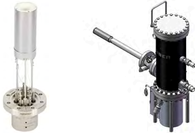
Figure 3.6: Effusion cell (left) and cracker cell (right). ( http://www.riber.com )
