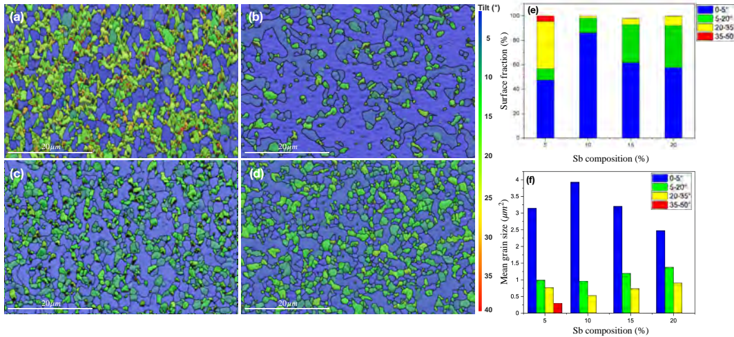
Figure 4.6: Determination of the grain orientation. EBSD map showing the angular deviation between the (0001) (a) Bi_{0.95}Sb_{0.05} , (b) Bi_{0.9}Sb_{0.1} , (c) Bi_{0.85}Sb_{0.15} , (d) Bi_{0.8}Sb_{0.2} grains and the GaAs(001) substrate. The colour scale corresponds to the tilt ranging from 0 to 40^\circ with respect to the substrate direction. (e) and (f) Statistics about the grain tilting angle and the grain size as a function of the antimony composition.
