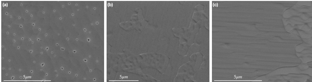
Figure 5.8: Determination of the surface morphology of 300 nm-thick \text{Bi}_{0.9}\text{Sb}_{0.1} films deposited on a \text{GaAs}(111)\text{A} substrate with a growth rate of (a) 0.4 \mu\text{m}/\text{h} , (b) 0.26 \mu\text{m}/\text{h} and (c) 0.13 \mu\text{m}/\text{h} .
