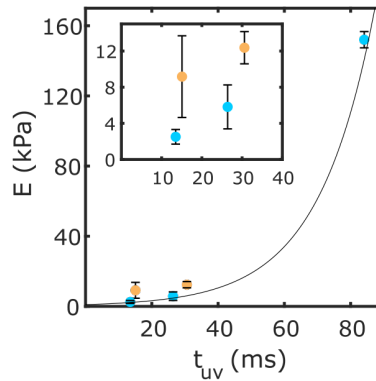
Figure 3.24: AFM measurements: Young's modulus increases exponentially with exposure time.
