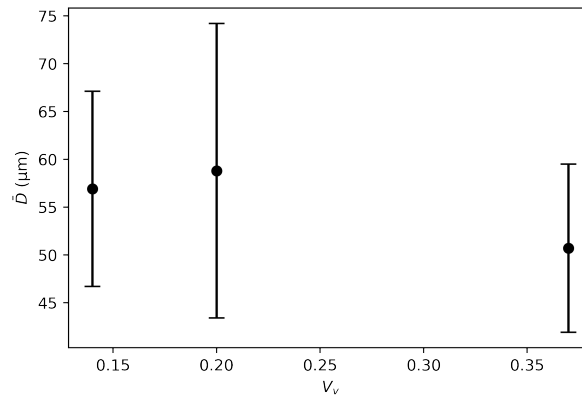
Fig. 4.16 Mean ( \bar{D} ) and standard deviation (error bars) in droplet diameter at the outlet of the hexagonal porous medium for various volume fractions of the dispersed phase with respect to the total dispersion volume ( V_v ).
