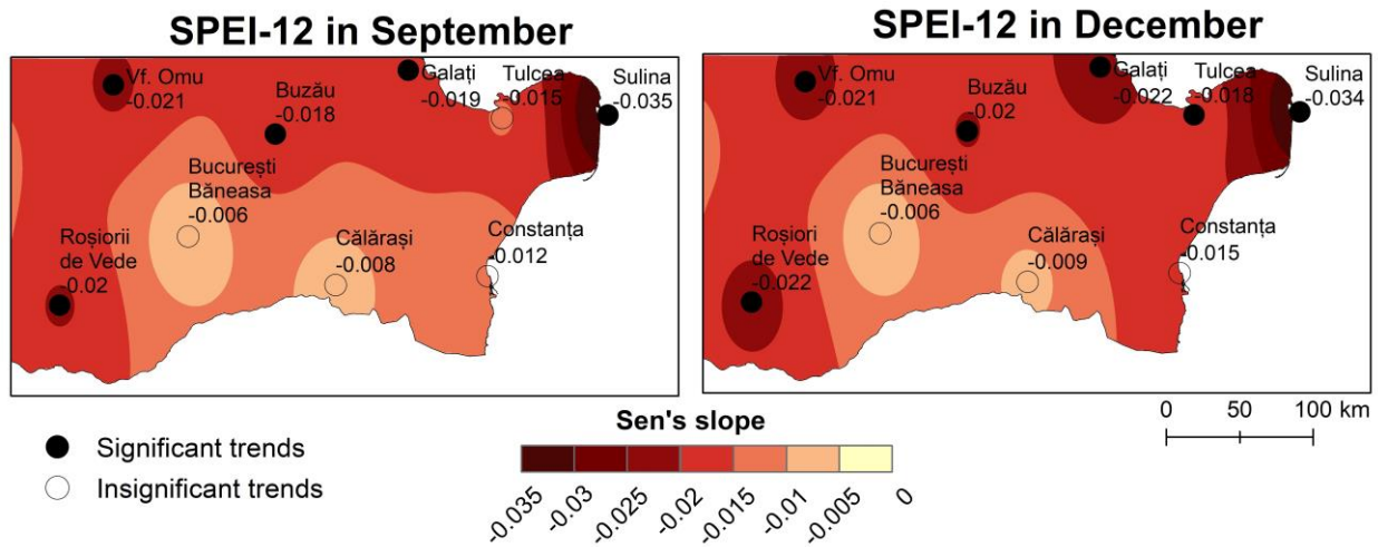
Figure 5.26 SPEI-12 trends in December and September over the 1961 – 2020 period
