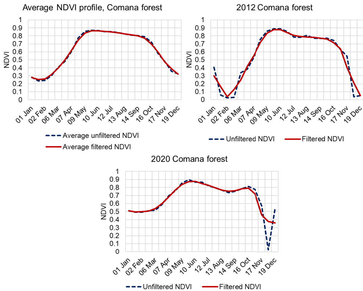
Figure 6.4 Comparison between raw NDVI and NDVI filtered with the Savitzky-Golay filter in the Comana Forest
