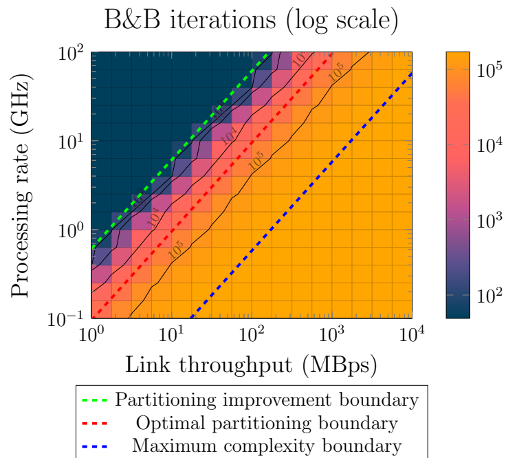
(b) B&amp;B complexity
