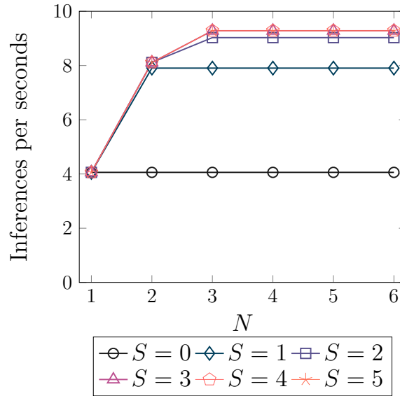
(a) B&B inference throughput
