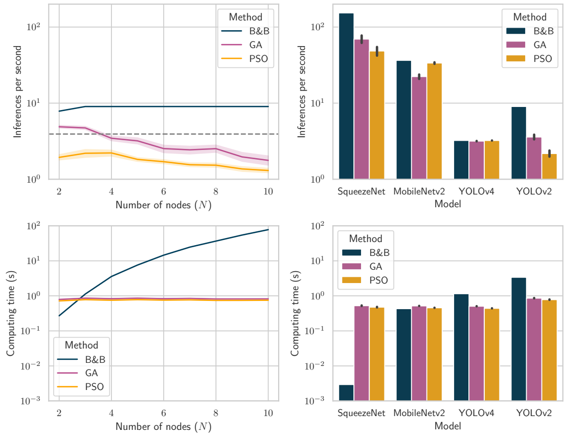
Figure 5.6: Comparative analysis of Branch and Bound (B&B), Genetic Algorithm (GA), and Particle Swarm Optimization (PSO), on the DNN partitioning problem to maximize the inference throughput.
