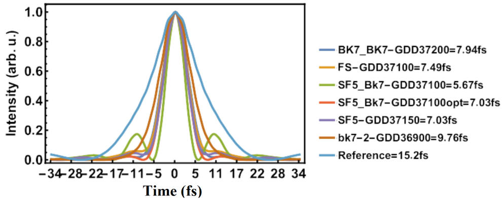
Figure 4.33: Fourier-limited pulses obtained from the spectra for each material.
