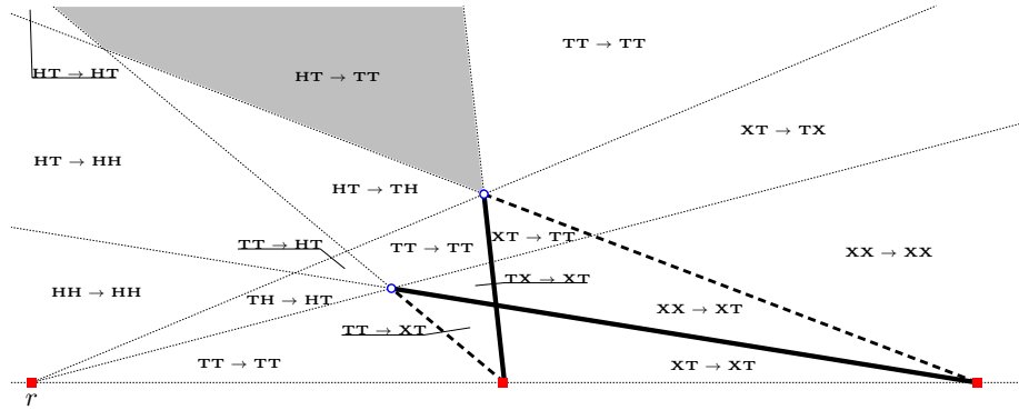
Figure 5.16: The case 1 “map” of all the possible red-on-a-line tracking choices. Tracking choices cannot avoid the transition H \rightarrow T in the shaded region.
