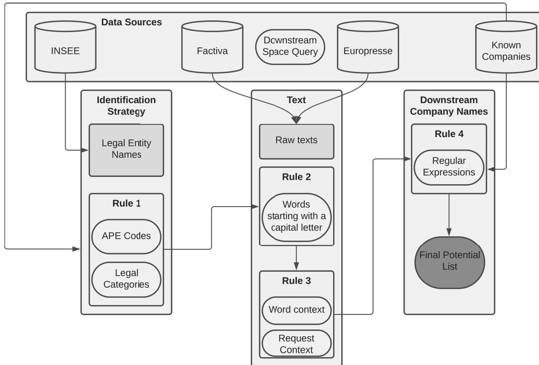
Figure 3.1: Rule-based strategy
