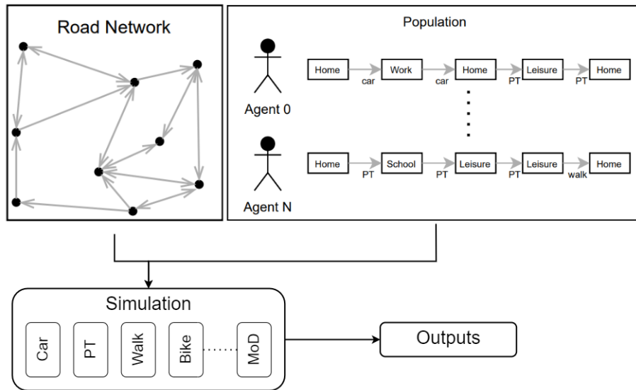
Figure 2.1: Overview of MATSim
