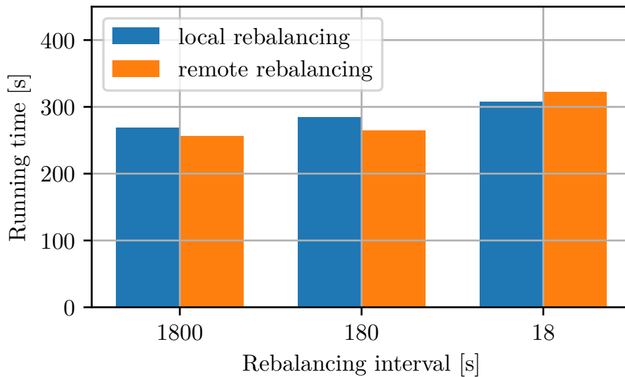
Figure 5.4: Communication overhead benchmark
