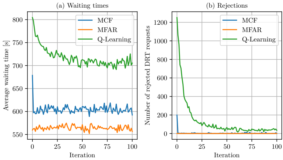
Figure 5.6: Comparison of between the implemented Q-learning algorithm and the MCF and MFAR algorithms. Figure 5.6.a shows the evolution of the average waiting time of performed DRT requests across the iterations of the simulation. Figure 5.6.b shows the evolution of the number of rejected DRT requests across the iterations of the simulation
