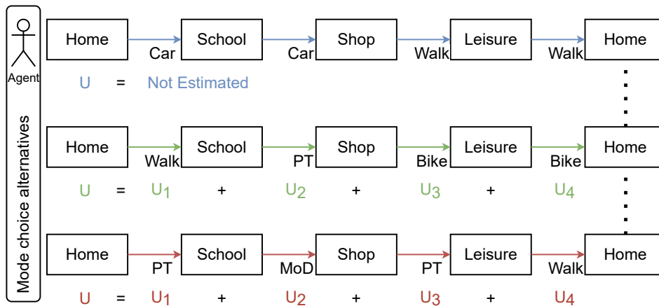
Figure 2.2: Summary of the DMC model implemented in MATSim. For a tour starting at ending at the activity type "home", All possible mode sequences are considered. In this example, the utility of the top alternative is not evaluated due to breaking the constraint that states that the car must be at the home location at the end of the tour
