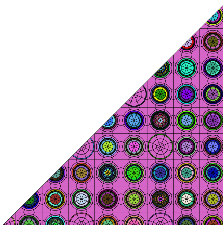
Figure 4.14: Mesh used for PWR \text{UO}_2 Fuel Assembly Calculation.
