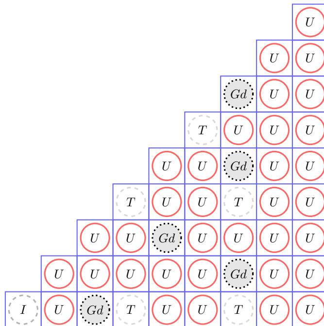
Figure 4.13: PWR \text{UO}_2 fuel assembly 1/8th geometry layout, with \text{UO}_2 fuel rod (U), gadolinium pins (Gd), RCC guide thimble (T) and instrumentation thimble (I).
