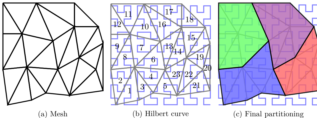
Figure 6.6: Geometric partitioning using Hilbert space-filling curve.
