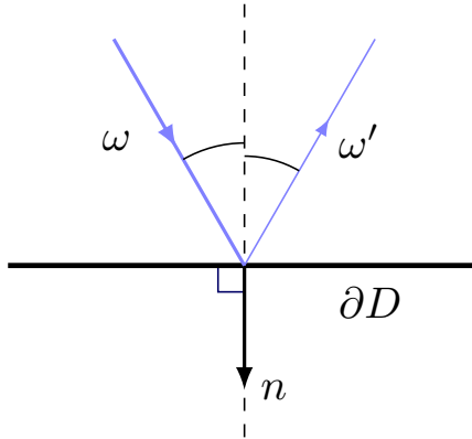
Figure 1.5: Specular reflection.
