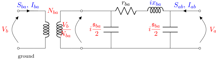
Figure 3: The \pi -model of a line \ell = (b, a) \in \mathcal{L} (from [28], courtesy of L. Liberti)
