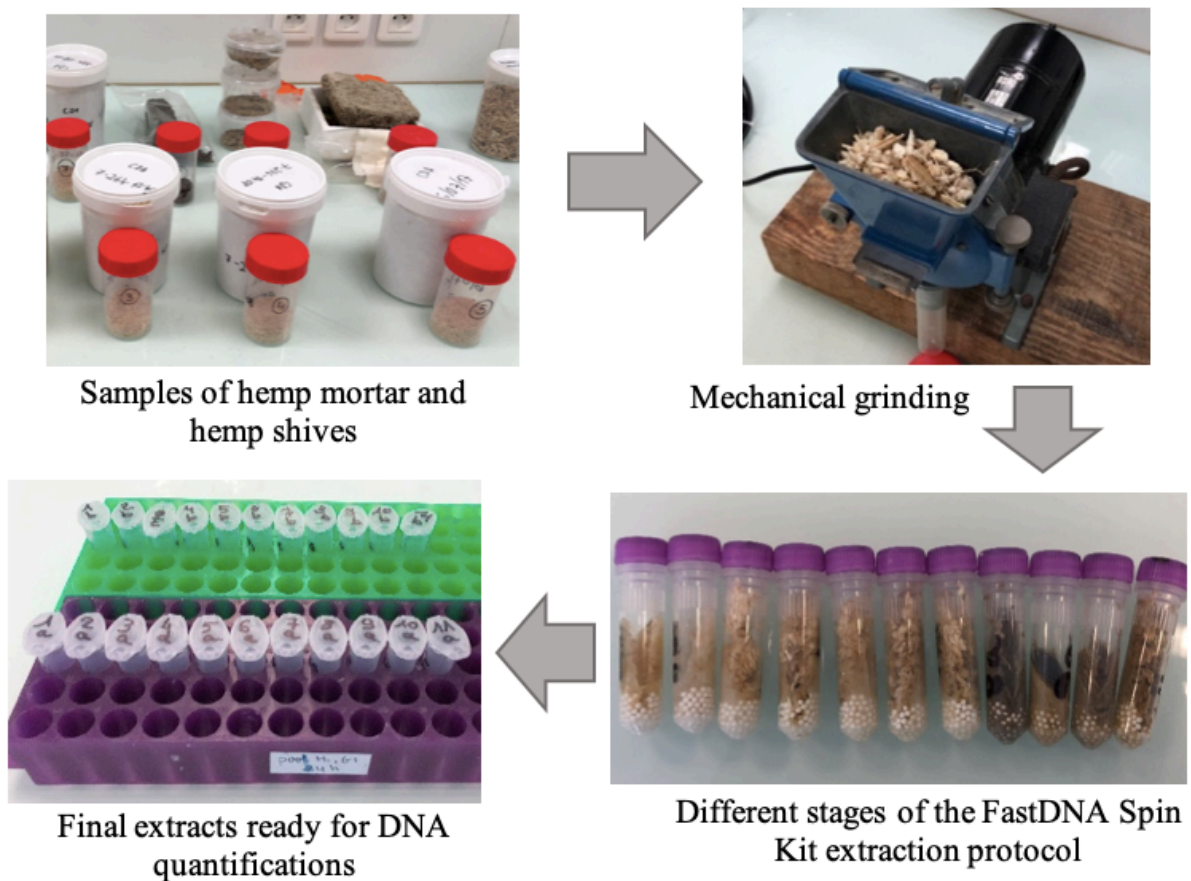
Figure 97. DNA extraction protocol schema
