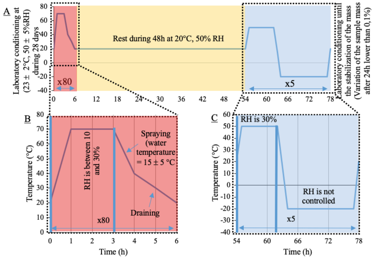
Figure 44. Diagram of the total accelerated aging cycles (A) with detailed heat-rain (B) and heat-cold (C) cycles
