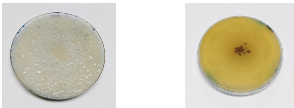
Figure 87. Image of Petri dish with isolated white fungal strain (identified as Rhizopus sp. ) after 8 days at 25 °C and 50 %RH
