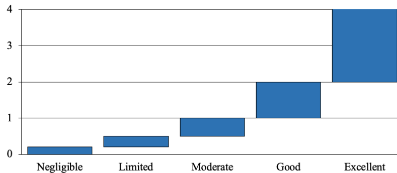
Figure 54. Moisture buffer value (g/%RH.m 2 ) standardization according to Nordtest protocol (NORDTEST project, 2005)
