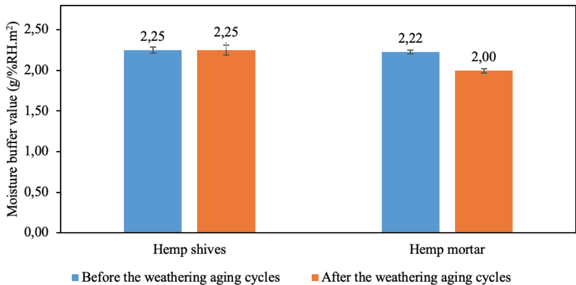
Figure 64. Moisture buffer value ( \text{g}/\%RH.m^2 ) evolution of hemp shives and hemp mortar samples before and after the accelerated aging cycles
