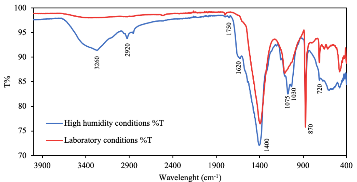
Figure 71. ATR-FTIR spectra obtained from hemp mortar samples conditioned during two years at high humidity and laboratory conditions
