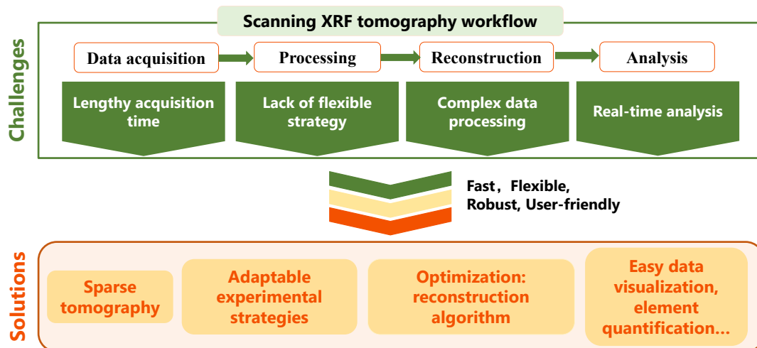
Figure 4.1: Challenges in scanning XRF tomography and proposed solutions. By integrating these proposed solutions into a coherent workflow, users can effectively overcome the challenges, making the technique more accessible and efficient for scientific applications.
