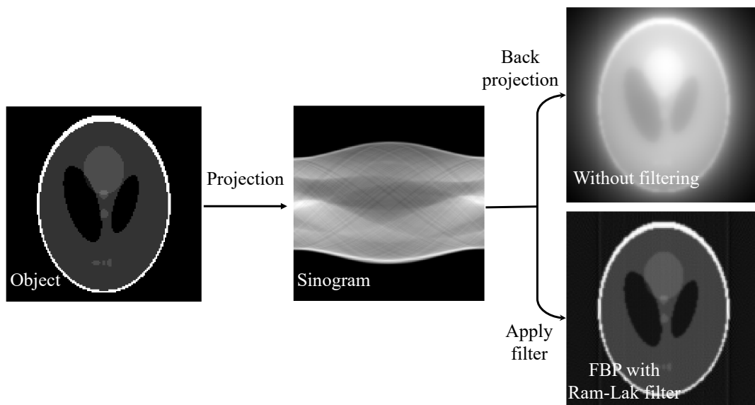
Figure 3.8: Reconstruction by FBP algorithm. Reconstruction of a Shepp-Logan phantom respectively by unfiltered back projection and FBP with Ram-Lak filter with 180 projections over 180^\circ .
