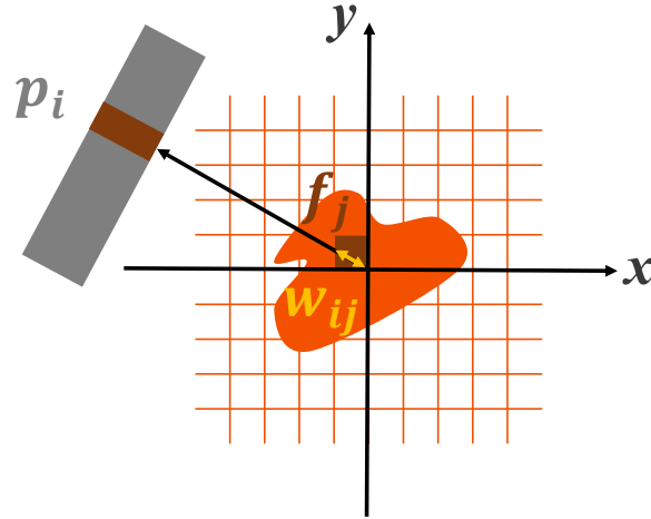
Figure 3.13: Illustration of the discretization of the projection process. The contribution w_{ij} of pixel j to the projection value p_i is illustrated as the length of intersection indicated in yellow.
