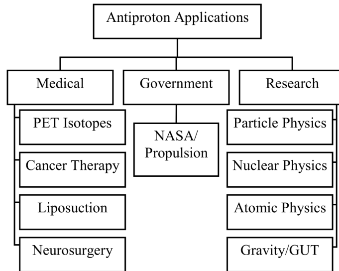
Figure 2.5: Diagram of the various categories of antiproton applications. The strongest commercial possibilities are in the field of medicine [Jac02].
