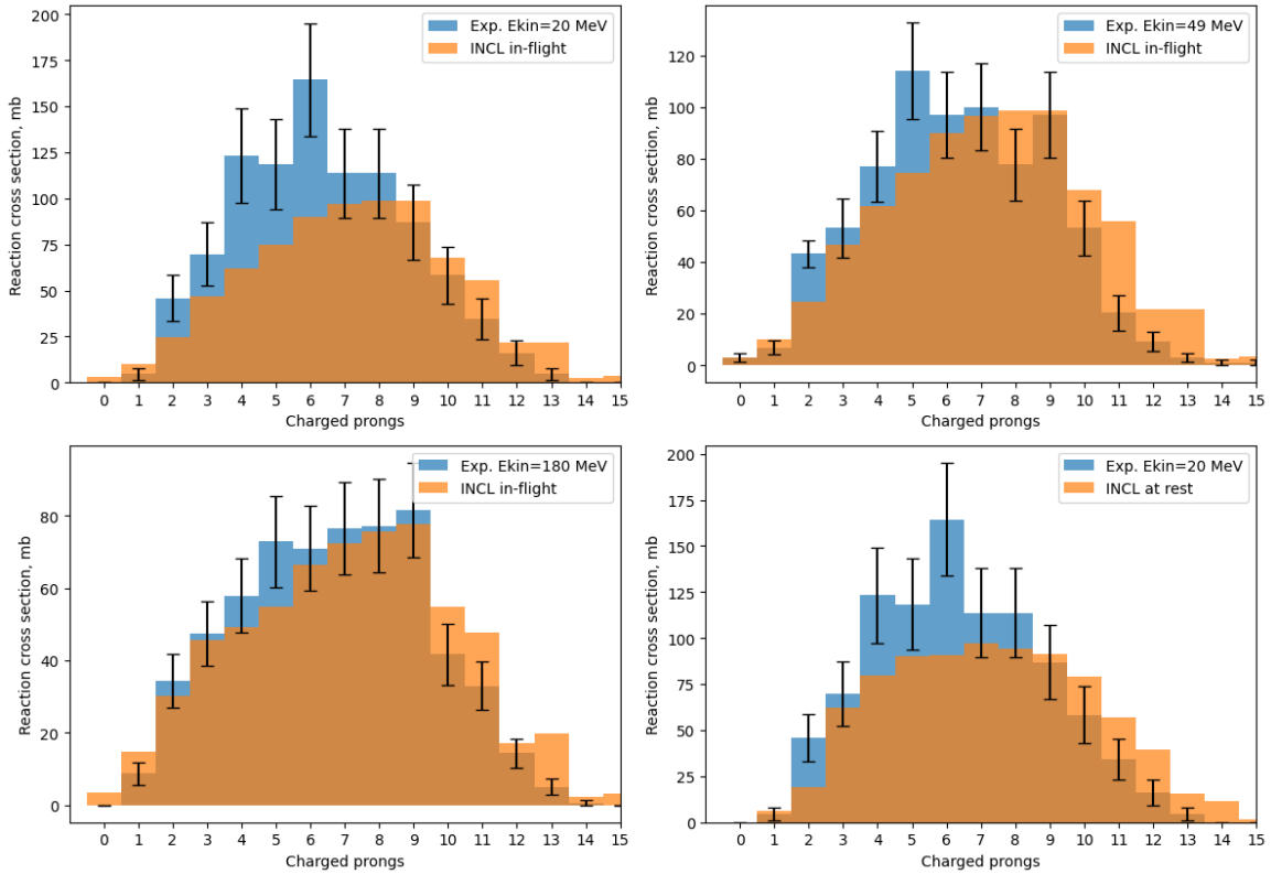
Figure 6.4: Charged prong multiplicity distributions for E_{kin} = 20, 49 and 180 MeV, the corresponding numbers of observed events are 956 \pm 47 , 771 \pm 28 and 623 \pm 21 . The systematic error is added directly to the statistical one, and was claimed to be 7% by the authors in Ref. [Bal+91].
