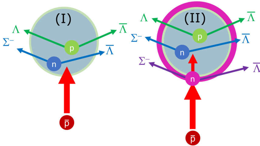
Figure 2.4: \Lambda\bar{\Lambda} and \Sigma^-\bar{\Lambda} pair production in antiproton–nucleus interactions, I and II denote two isotopes, where the heavier one (II) has additional neutron thickness. Taken from [Chr+22].
