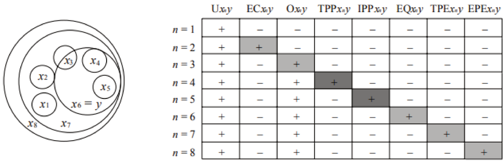
FIGURE 3.5 – The basic mereotopological relations, with shaded cells indicate connection and darker shading tands for parthood. Source : Figure from Achille C. Varzi in [Varzi2007].
