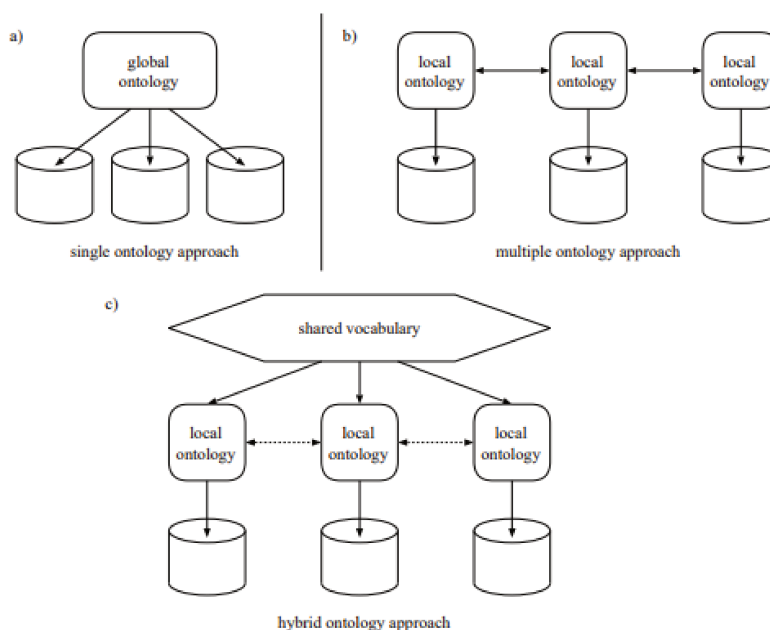
FIGURE 1.8 – The three possible ways for using ontologies for content explication. Source : Figure from Holger Wache et al. in [Wache2001].
