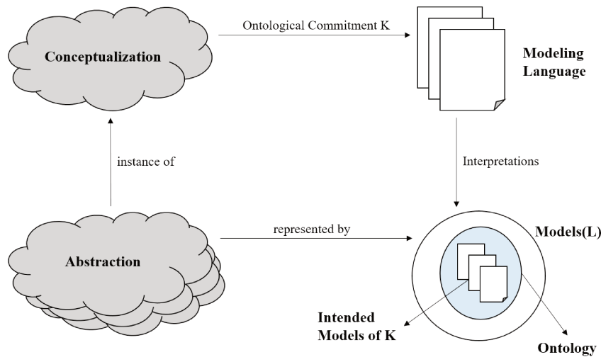
FIGURE 1.5 – The relationships between Abstractions, their Conceptualization, the Modeling Language, its Intended models, and an Ontology. Figure adapted from the figure proposed by Nicola Guarino in [Guarino2009b].
