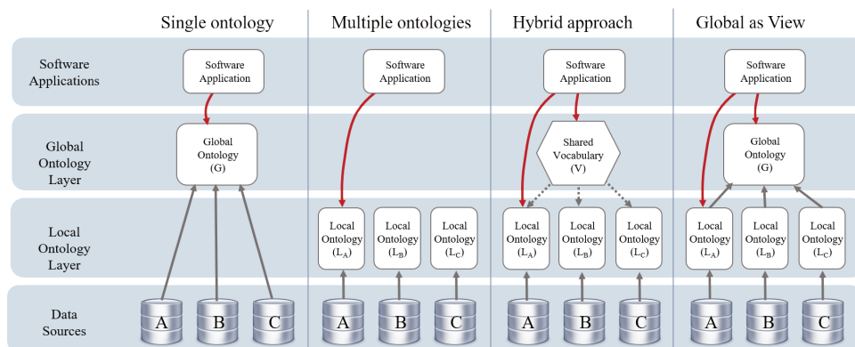
FIGURE 1.10 – Three variants of OBDI : (1) single-ontology, (2) multiple-ontology, (3) hybrid, and an additional OBDI variant (4) Global-as-View (GaV). Source : Figure adapted from Fajar J. Ekaputra et al. [Ekaputra2017].
