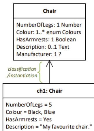
FIGURE 2.14 – A snapshot of ConML’s (version 1.5) Basic Graphical Notation Summary depicting the instantiation relationship between an individual and a class. Source : http://www.conml.org/Resources/Training.aspx .
