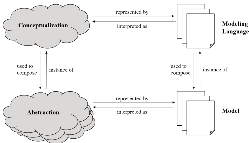
FIGURE 1.4 – Relations between Conceptualization, Abstraction, Modeling Language, and Model. Source : Figure from Giancarlo Guizzardi in [Guizzardi2007].
