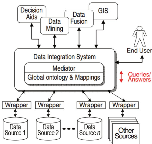
FIGURE 1.9 – An Ontology-Based Data Integration Architecture. Source : Figure from Michel Gagnon in [Gagnon2007].
