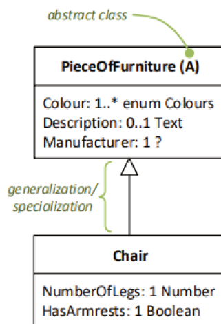
FIGURE 2.13 – A snapshot of ConML’s (version 1.5) Basic Graphical Notation Summary showing the generalization/specialization relationship between two classes. Source : http://www.conml.org/Resources/Training.aspx .
