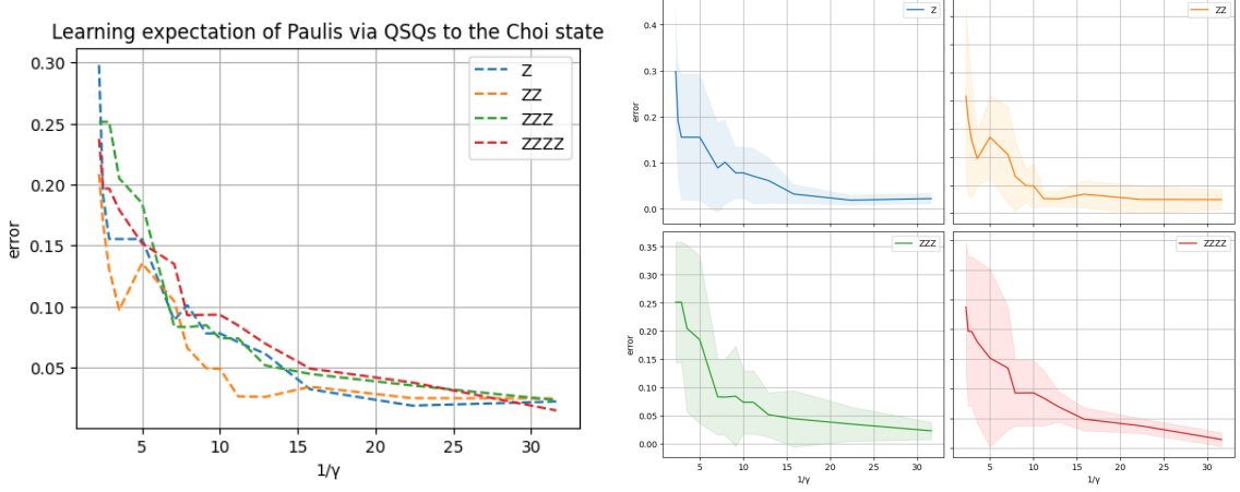
Figure 6.1: Average performance of the Goldreich-Levin algorithm implemented with quantum statistical queries to the Choi-Jamiolkowski state. We tested the algorithm on 10 random 4-qubit random unitaries, in predicting the absolute value of the outcome of Z observables on the unitary evolution of computational basis states. Each random unitary consists in 2 layers of Haar-random gates. We plotted the average error as a function of 1/\gamma , i.e. the inverse of the threshold of Algorithm 2. We set the tolerance of the quantum statistical queries as \gamma^2/4 .
