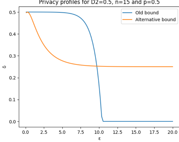
Figure 8.1: In this figure we compare the former upper bound from [HRF23] (Equation 8.30) with the novel upper bound provided in this section (Equation 8.31). We emphasise that each bound outperforms the other for some values of \epsilon . We assumed that the input state satisfy D_2(\rho \| I/2^n) \leq 0.5 , n = 15 and p = 0.5 . The upper bound on \tau is derived from \|\rho - \sigma\|_1 \leq \|\rho - I/2^n\|_1 + \|\sigma - I/2^n\|_1 \leq 2\sqrt{2D_2(\rho \| I/2^n)} , i.e. combining the triangle inequality and the Pinsker's inequality.
