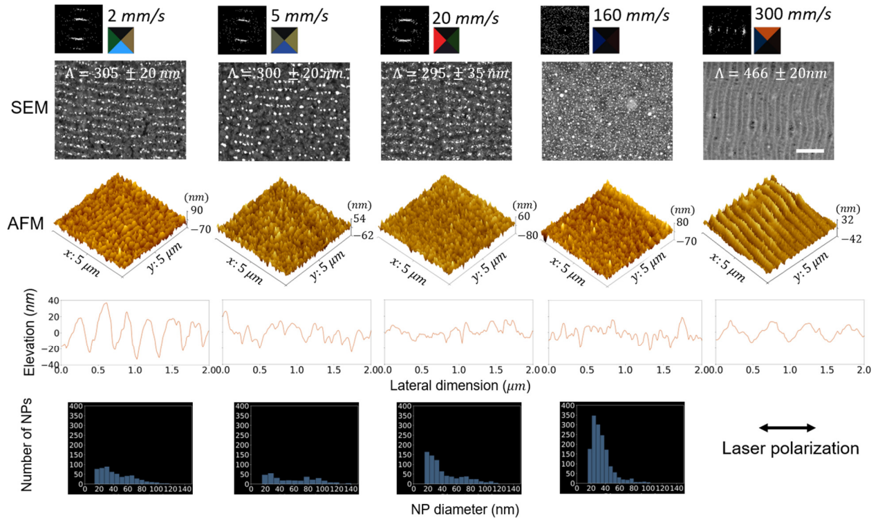
Fig. 4.2. (a) Evolution of the physical and optical properties of laser-induced metasurfaces when varying the scan speed (from 2 \text{ mm}\cdot\text{s}^{-1} to 300 \text{ mm}\cdot\text{s}^{-1} ) at low fluence ( 87 \text{ mJ}\cdot\text{cm}^{-2} ), high repetition rate ( 600 \text{ kHz} ) and large overlapping between laser lines ( dy = 2 \mu\text{m} ). For each scan speed, the sample is characterized by a four-color chart (as described in Figure 4.1), a representative scanning electron microscopy (SEM) image with the value of the grating period and its Fourier transform on the top corner left, an atomic force microscopy (AFM) 3D view of the surface topography and the corresponding surface profile, measured along the x axis for the 4 left images and along the y axis for the sample at 300 \text{ mm}\cdot\text{s}^{-1} , and a histogram of the nanoparticle sizes as observed by SEM. The double arrow indicates laser polarization for the SEM images. The scale bar is 1 \mu\text{m} in all SEM images.
