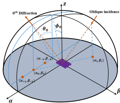
Fig. 5.1. Positions of incidence and diffraction orders in direction cosine space denoted as \alpha , \beta which the subscript “i” for incidence, “0” for 0 th diffraction orders, “+1” for +1 st diffraction orders, and “-1” for -1 st diffraction orders.
