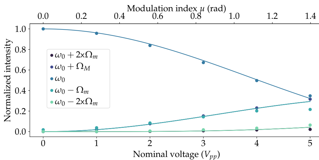
Figure B.2: Characterization of the electro-optic 188-44-13, with a measured V_{\pi} = 11.237 V_{PP}
