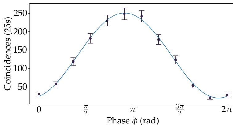
Figure 4.24: Two photon interferences for frequency-entangled qubits. The experimental points (dot) are fitted with a sine curve (refer to text).
