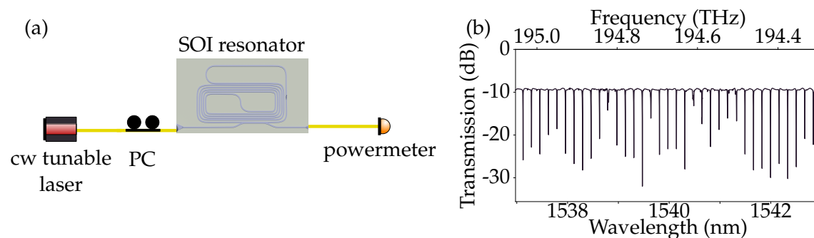
Figure 2.11: (a): Experimental setup and (b): Measured transmission spectrum of the cavity.
