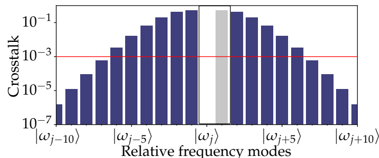
Figure 3.7: Probability distribution of a photon initially in |\omega_j\rangle after a bit-flip gate. The horizontal red line corresponds to a crosstalk threshold of 10^{-3} .
