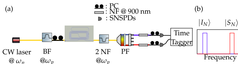
Figure 2.16: (a): Setup for detecting single counts and coincidences from the SOI microresonator. BP: bandpass filter, NF: notch filter, PC: polarization controller. (b): The programmable filter applies two 21 GHz bandpass filters to select specific signal and idler mode |I_N\rangle and |S_N\rangle . The two photons are then spatially separated into two distinct fibers.
