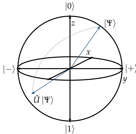
Figure 3.1: Representation on the Bloch sphere of the action of a single qubit rotation \hat{U} on an input single qubit state |\Psi\rangle . |+\rangle and |-\rangle are the superposition states defined as |+\rangle = |0\rangle + |1\rangle and |-\rangle = |0\rangle - |1\rangle
