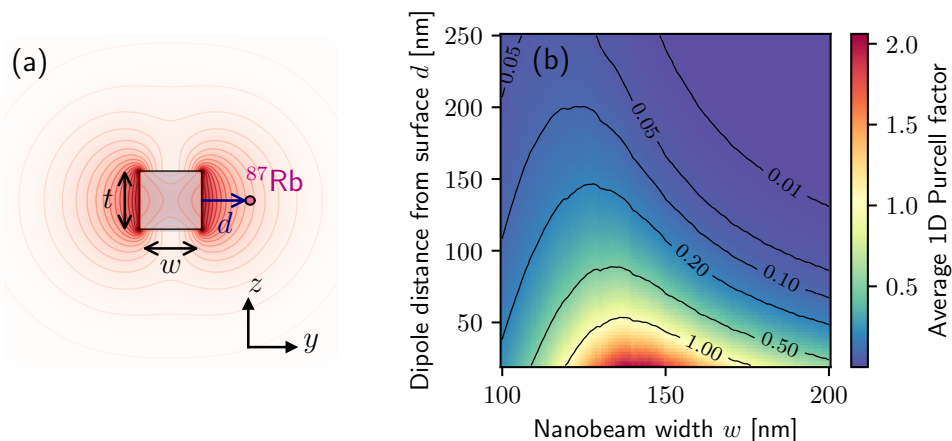
Figure 5.1: Optimization of the width of a suspended nanobeam. (a) Scheme of the transverse plane of a nanobeam, defined by its width w and thickness t . The contour plot shows the transverse intensity profile of a propagating TE-like mode. The nanobeam is made of GaInP ( n = 3.35 ) (b) Average 1D Purcell factor \Gamma_{1D}/\Gamma_0 depending on the width of the nanobeam and the distance of the atom. \Gamma_{1D}/\Gamma_0 around 0.1 – 0.2 are expected for nanobeams with w = 140 nm and realistic atom trap distances (see main text). The thickness t is fixed to t = 150 nm.
