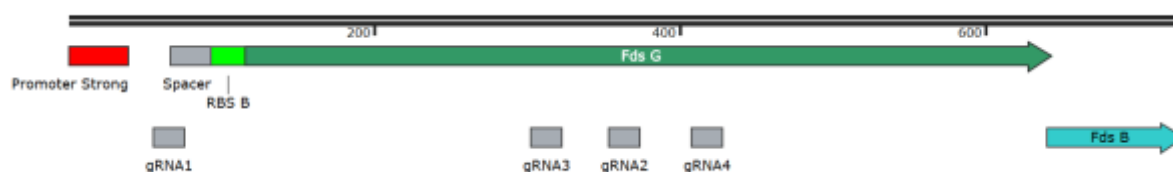
Figure 43. Representation of the positions targeted by the four gRNAs selected for CRISPRi gene silencing.
