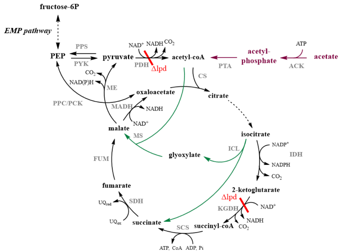
Figure 26. E. coli \Delta lpd strain metabolism. The red bars represent the lpd gene disruption. ACK, acetate kinase; CS, citrate synthase; FUM, fumarase; IDH, isocitrate dehydrogenase; KGDH, 2-ketoglutarate dehydrogenase complex; MADH, malate dehydrogenase; ME, malic enzymes; MS, malate synthase; PDH, pyruvate dehydrogenase; PCK, PEP carboxykinase; PPC, PEP carboxylase; PPS, PEP synthetase; PTA, phosphate acetyltransferase; PYK, pyruvate kinase; SCS, succinyl-CoA synthetase; SDH, succinate dehydrogenase. Redesigned from Wenk et al. (2020).
