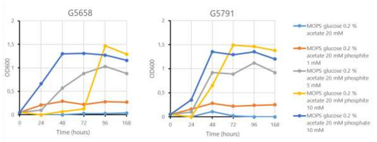
Figure 59. Growth of strains G5658 ( \Delta phoA \Delta phnI \Delta lpd ) and G5791 ( \Delta phoA \Delta phnI \Delta lpd kdgK::ptxD ) within a range of phosphite concentrations from 1 to 10 mM. Strains were grown in MOPS mineral medium supplemented with glucose 0.2 % acetate 20 mM medium supplemented with the indicated concentration of phosphite ranging from 0 to 10 mM.
