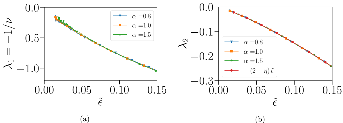
Figure 4.1 – LPA': Numerical results above d_{lc} for the two relevant eigenvalues, calculated with the exponential regulator. The prediction \lambda_2 = -(2-\eta)\tilde{\epsilon} is also displayed in the right panel. Markers are plotted for every 30th data point.
