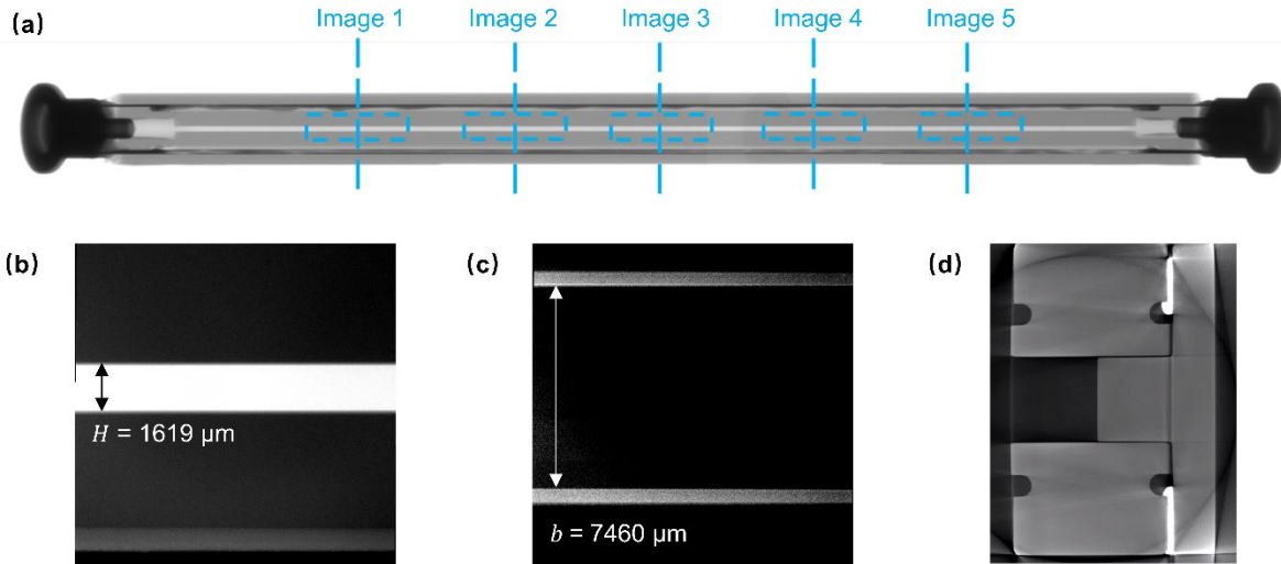
Figure 5.4. Tomography image of the channel. (a) The whole channel in the view of ICCD, each pixel represents 85.62 μm; (b) Measurement of the channel height, each pixel represents 7.71 μm; (c) Measurement of the channel width, each pixel represents 7.97 μm; (d) Cross-section of the channel.
