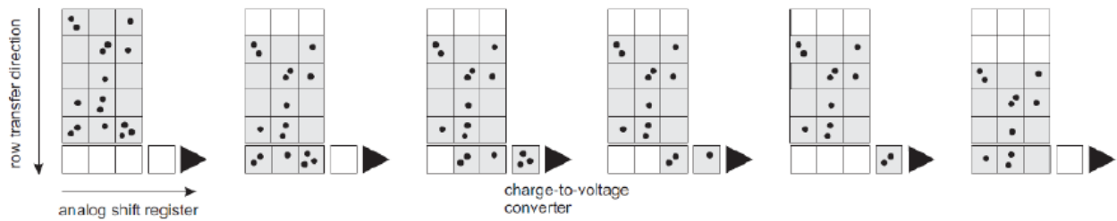
Figure 4.6. Readout process in each single cell of the CCD. Figure from LaVision® documentation.
