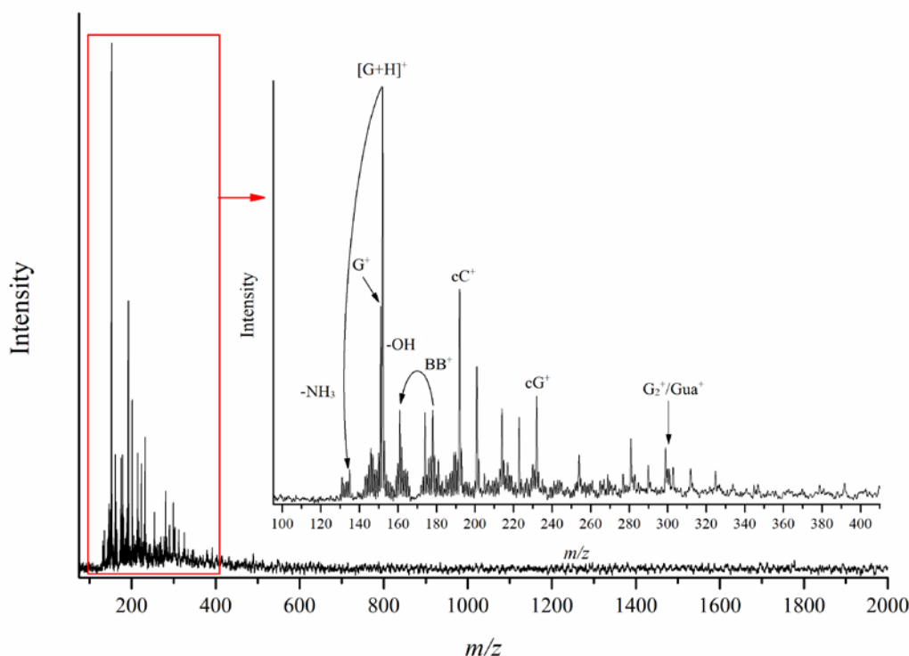
Figure 5.2: Mass spectrum of the positive products of [dCGCGGGCCCGCG-4H]^{4-} after irradiation by ^{13}C^{3+} carbon ions at 10.4 MeV kinetic energy for a trap RF voltage of 2000 V.
