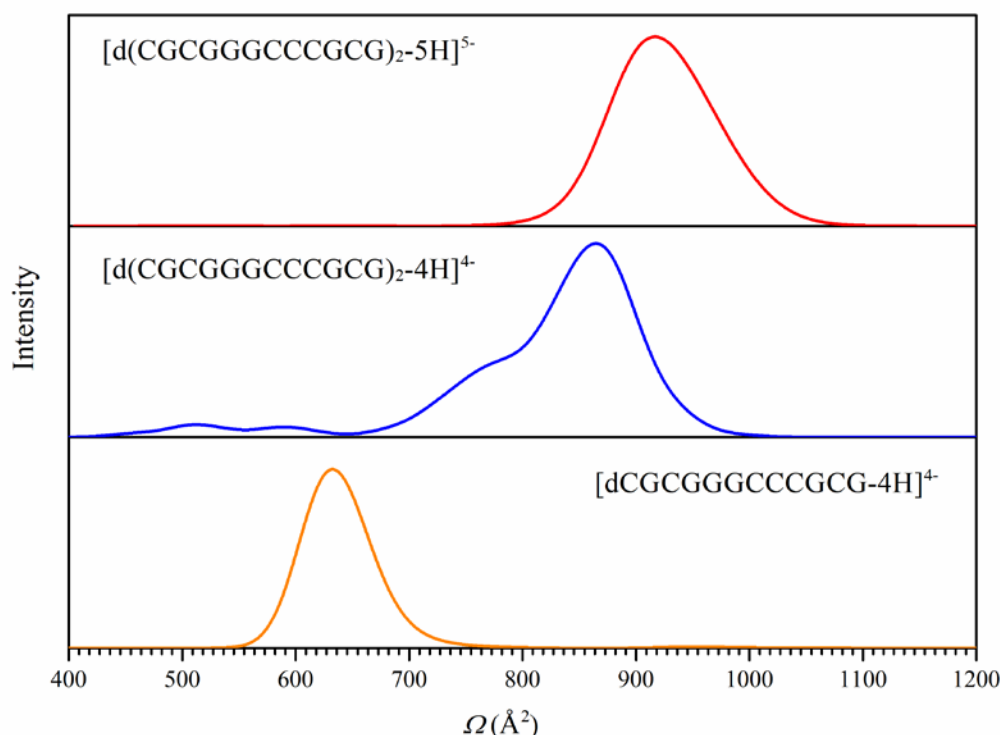
Figure 3.9: Experimental collision cross sections of [d(\text{CGCGGGCCCGCG})_2\text{-5H}]^{5-} , [d(\text{CGCGGGCCCGCG})_2\text{-4H}]^{4-} and [d\text{CGCGGGCCCGCG-4H}]^{4-} .
