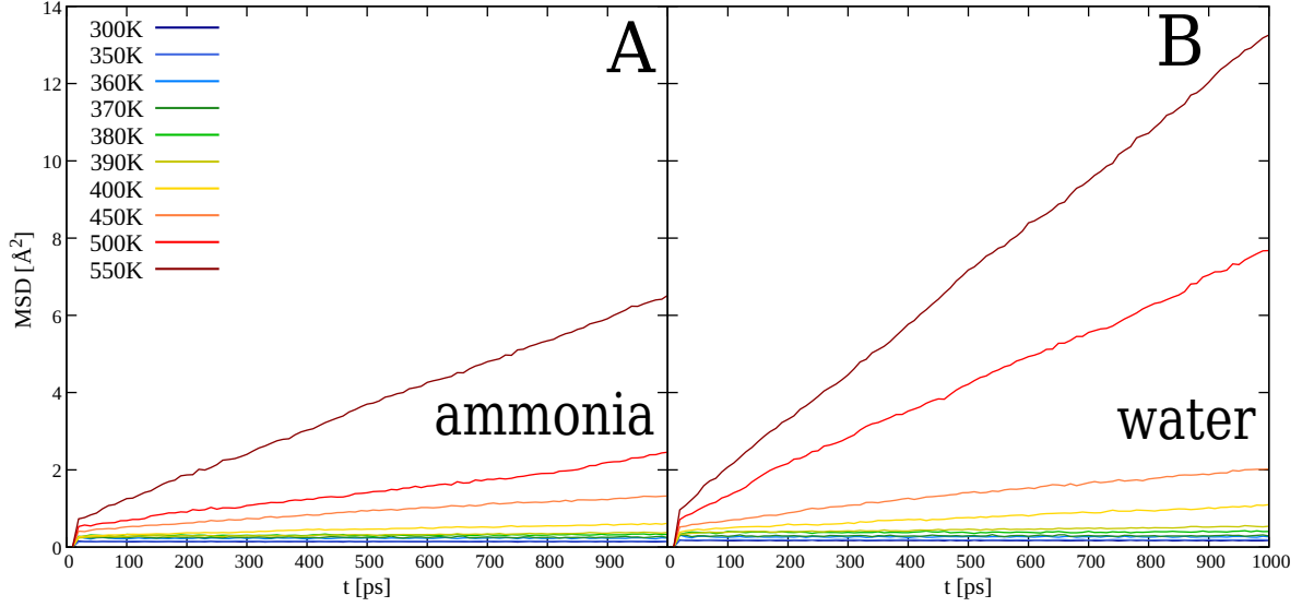
Figure 4.21: Mean squared displacement (MSD) of nitrogen atoms (panel A) and oxygen atoms (panel B) as function of time.
