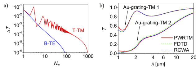
Fig. 2. a) Absolute value difference between transmittances calculated for 2000 plane waves and given numbers of plane waves ( N_w ) for B-TE (blue line) and T-TM (red line) configurations, b) transmittance calculated by FDTD (dashed line), RCWA (dotted line) and PWRTM (solid line) for a gold grating implemented on top of a substrate with a refractive index of 1.45 and the following parameters: L = 300 nm, a = 200 nm (Au-grating-TM 1) and L = 300 nm, a = 285 nm (Au-grating-TM 2).
