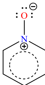
Figure V.2 1 : Chemical structure of pyridine N-oxide.
