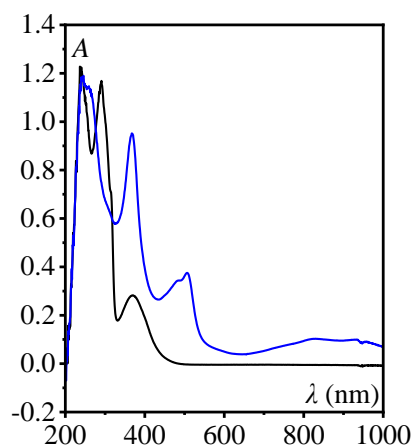
Figure V.3.3.4 7 : UV-vis spectrum of 1 mM [\text{Re}(\text{bpy})(\text{CO})_3\text{Cl}] + 500 \text{ mM H}_2\text{O} before electrolysis (black) and after E_{\text{app}} = -1.52 \text{ V} (blue) + 0.1 M \text{n-Bu}_4\text{NPF}_6 in \text{CH}_3\text{CN} .
