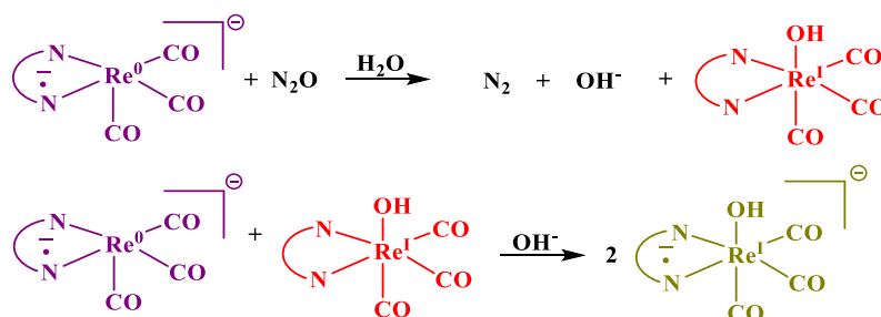
Scheme IV.3.3 1 : Proposed mechanism for the reaction of \text{N}_2\text{O} with the bi-reduced species [\text{Re}^0(\text{bpy}^{\bullet-})(\text{CO})_3]^- .
