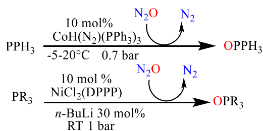
Scheme I.4.2.1 6 : Metal catalyzed oxidation of phosphines by N_2O .
