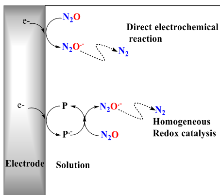
Figure II.5 1: Schematic representation of direct electrochemical reduction and homogeneous redox catalysis of N_2O .
