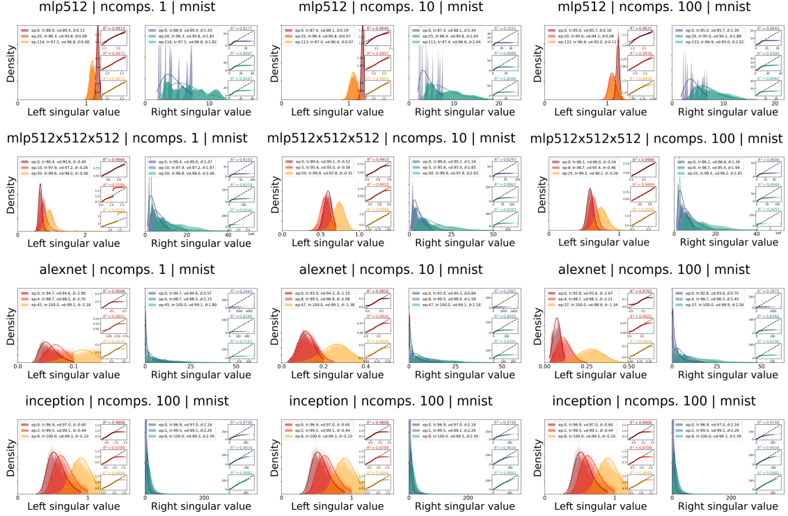
Figure 4.5: Point Jacobian spectral distribution for model | nbr. pca comp. | MNIST , from first epoch to overfit. "Left" and "right" distributions (cf. 4.5.3) are represented separately for each triplet for clarity. The best fit lognormal plot is superimposed on each histogram, with the corresponding probability plot on the right, with the line of best fit ( R^2 displayed on top). Legend elements, in order: epoch, training and validation accuracy, and the mean log spectrum.
