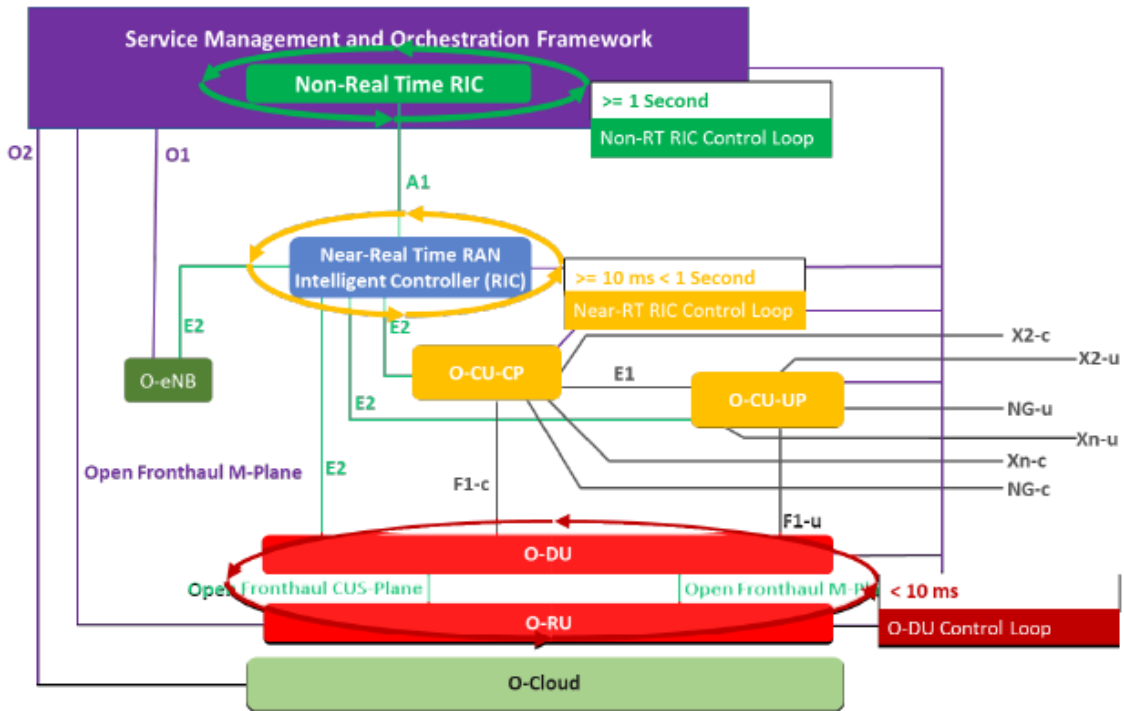
Figure 1.7: O-RAN Architecture [4]
