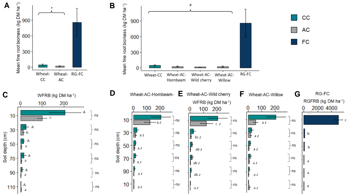
Figure 2: Mean values of wheat (WFRB, kg DM ha -1 ) and RG fine roots biomass (RGFRB, kg DM ha -1 ) in sole-crop control (CC), alley-cropping (AC) and pure-forest control (FC) plots. (A) Mean values for all data, (B) mean values according to the associated tree species, (C) mean values according to depth for Wheat-CC and Wheat-AC, (D) for Wheat-CC and Wheat-AC-Hornbeam association, (E) for Wheat-CC and Wheat-AC-Wild cherry association, (F) for Wheat-CC and Wheat-AC-Willow association and (G) for RG-FC association. Data are means ( \pm SE). In graphic (A), Asterisk indicates significant difference between type of system (Kruskal-Wallis’ test; p < 0.05 ). In graphic (B), symbol # indicates significant difference between wheat associated species and RG (Kruskal-Wallis’ test; p < 0.1 ). In graphics from (C) to (F), uppercase and lowercase letters (a, b and c) indicate homogeneous groups for comparison between soil layer for Wheat-CC and Wheat-AC, respectively (Tukey’s test; p < 0.05 ). In graphics (E), (F) and (G), italic letters (z) indicate homogeneous group to compare fine root of wheat in AC, associated with different tree species (Dunn’s test; p < 0.1 ). Symbols “ns” are result of Student’s test between the type of system (AC, CC) on fine root biomass for a given soil layer. “ns” means not significant. In graphic (E), lowercase letters indicate homogeneous groups for comparison between soil layer (Tukey’s test; p < 0.05 ).
