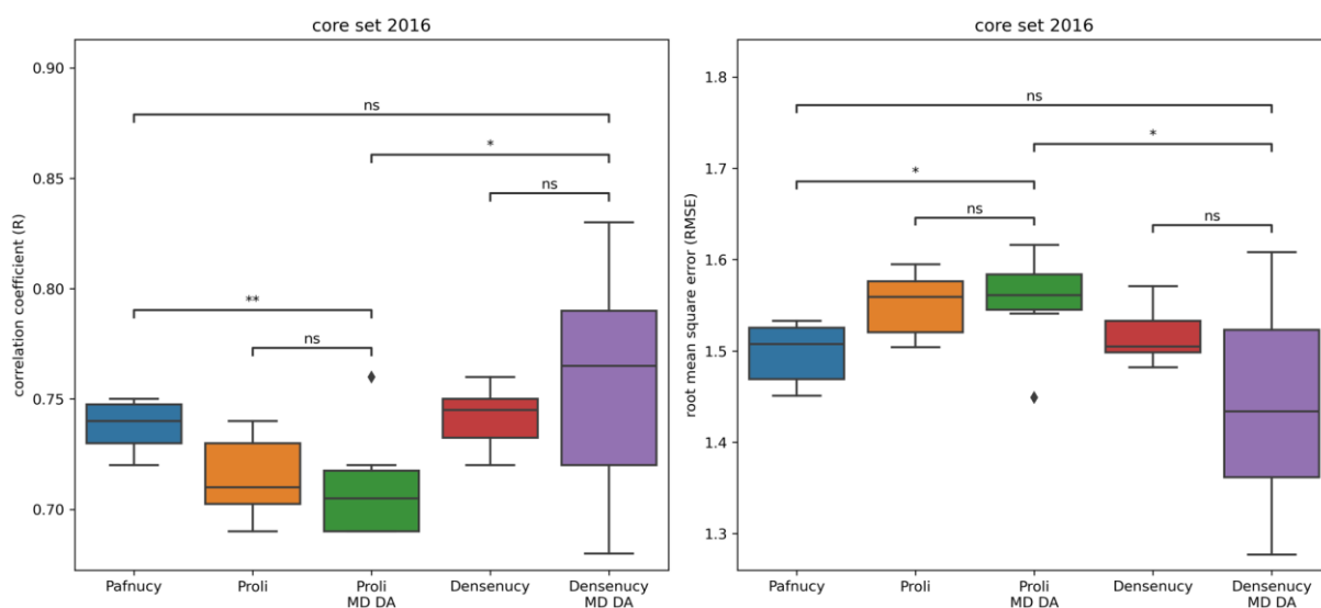
Figure 7. Comparison of the performance of Proli and Densenucy with or without data augmentation. Pafnucy performance without data augmentation on the same pockets was added for benchmark purpose. Results are evaluated on the PDBbind v.2016 core set. For each training setting, the boxplot displays the results over 10 replicate models. "MD DA" refers to molecular dynamics data augmentation. The following p-values correspond to the annotations on the plots: ns: 5.00 \times 10^{-2} < p \leq 1.00 \times 10^0 , *: 1.00 \times 10^{-2} < p \leq 5.00 \times 10^{-2} , **: 1.00 \times 10^{-3} < p \leq 1.00 \times 10^{-2} , and \blacklozenge are possible outliers.
