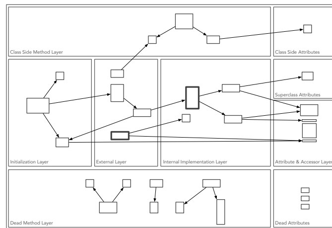
Figure 6.3: A colorless BLUEPRINTV2 with the graphical representations of methods, attributes, and accessors using height and width metrics. The arcs represent calls between methods and accesses to attributes.
